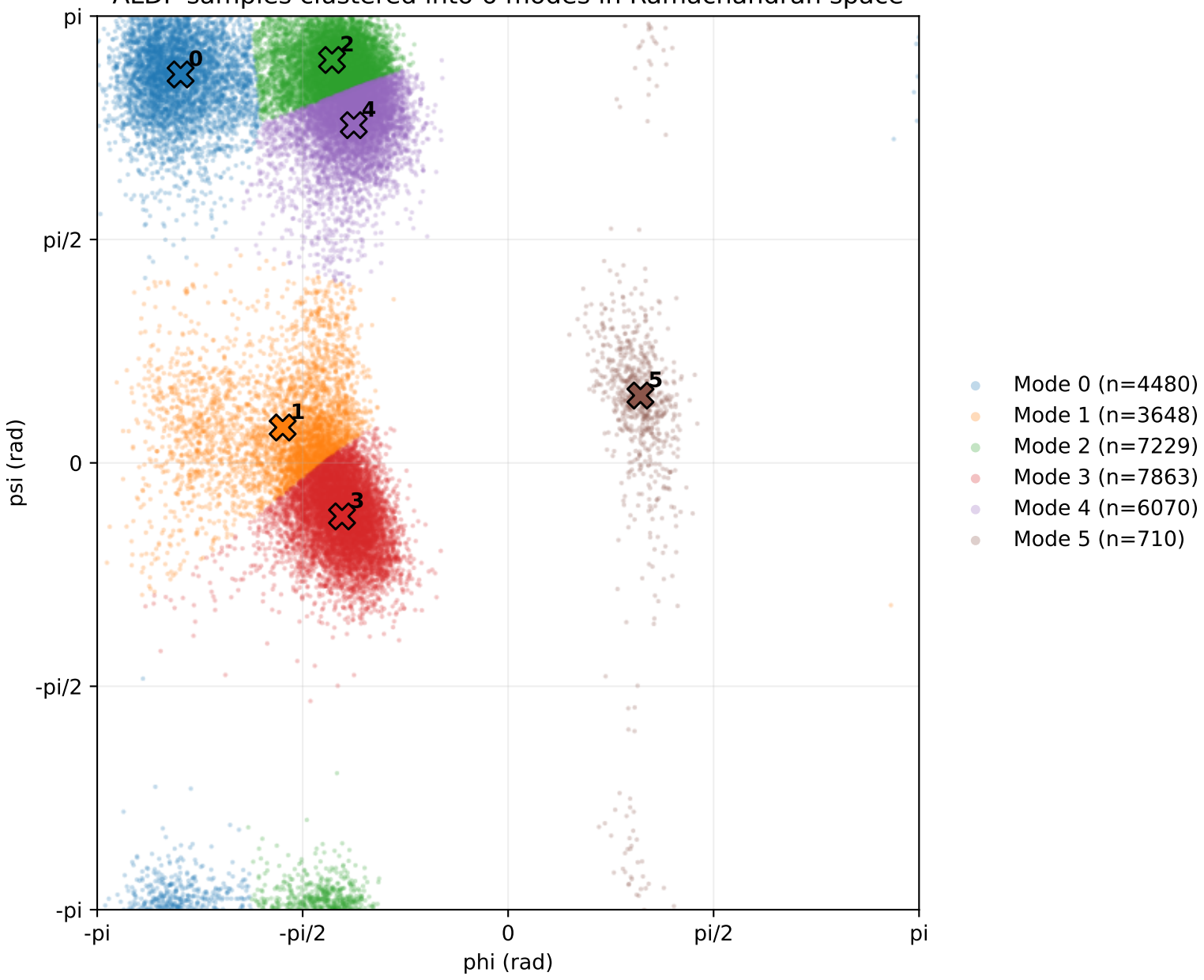
ALDP samples clustered into 6 modes in Ramachandran space
