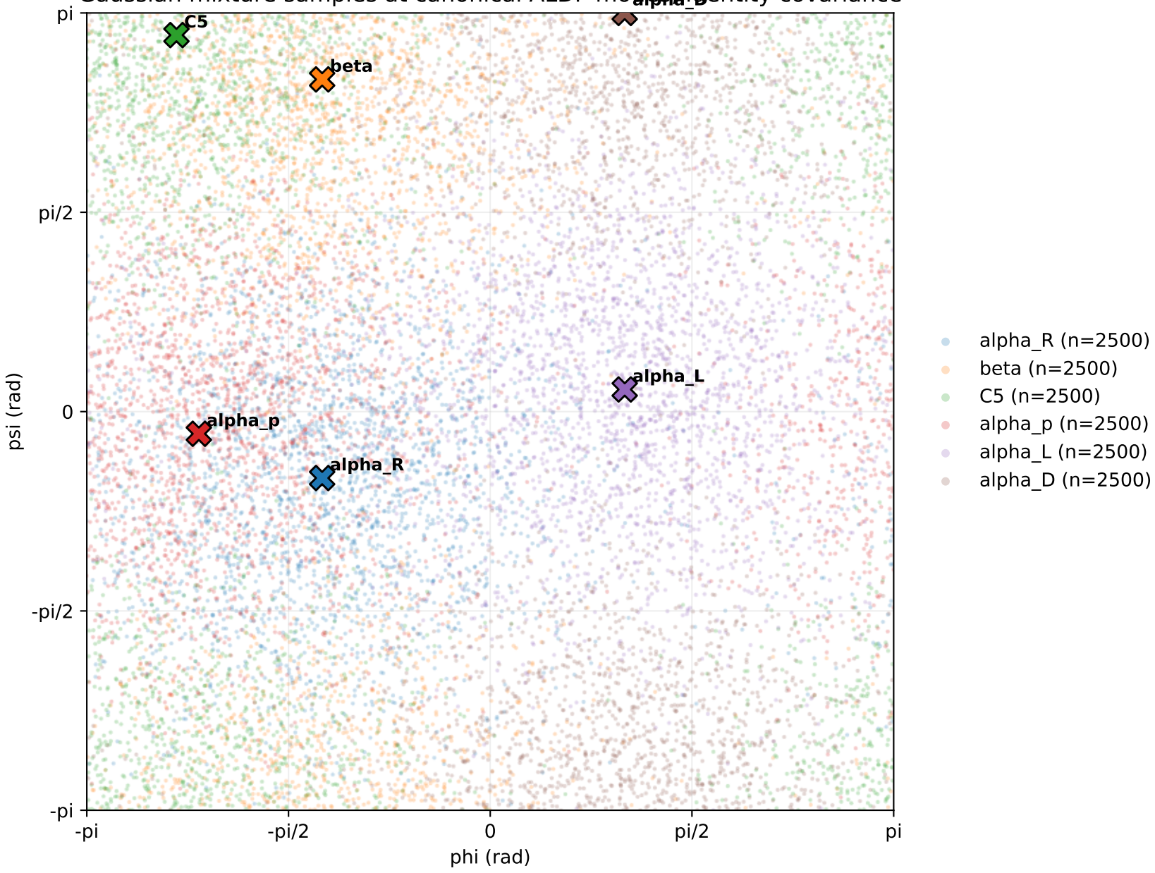
Gaussian mixture samples at canonical ALDP modes, identity covariance
