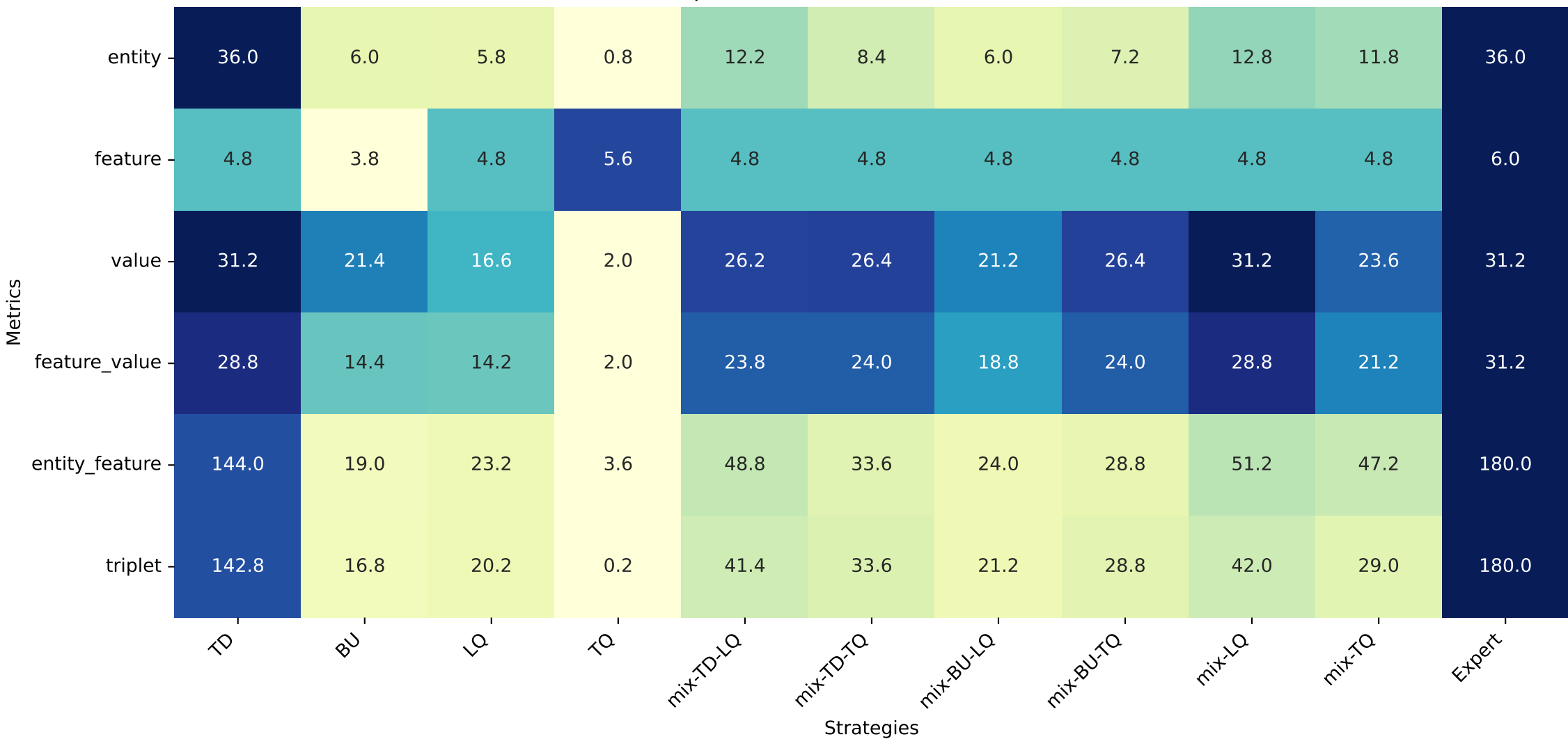
Heatmap of Correct Elements (Row-normalized)
