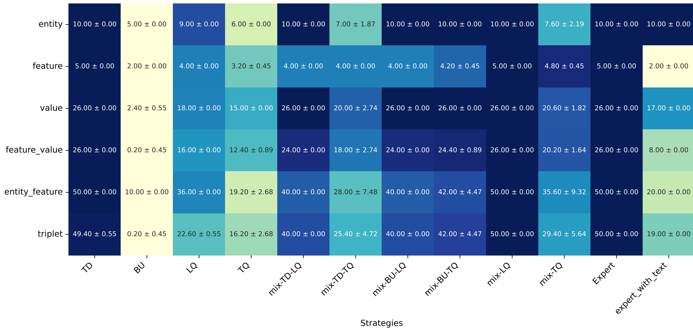
Heatmap of Correct Elements (mean \pm std, row-normalized)
