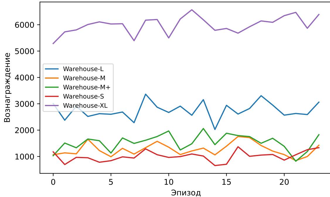
Q MIX Reward
