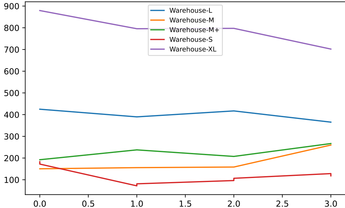
QMIX Reward
