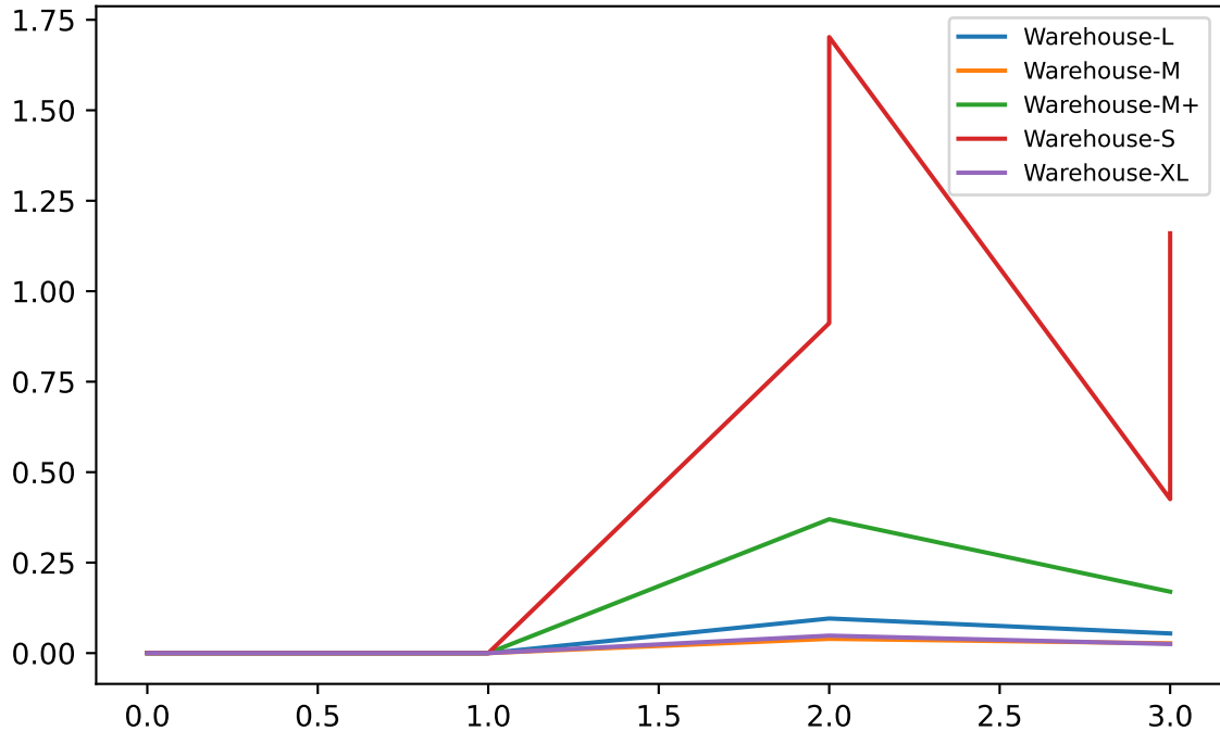
QMIX Loss
