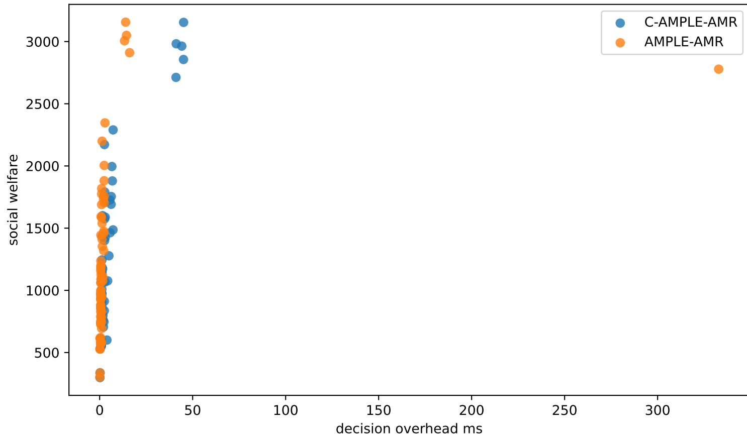
Global vs Clustered Tradeoff
