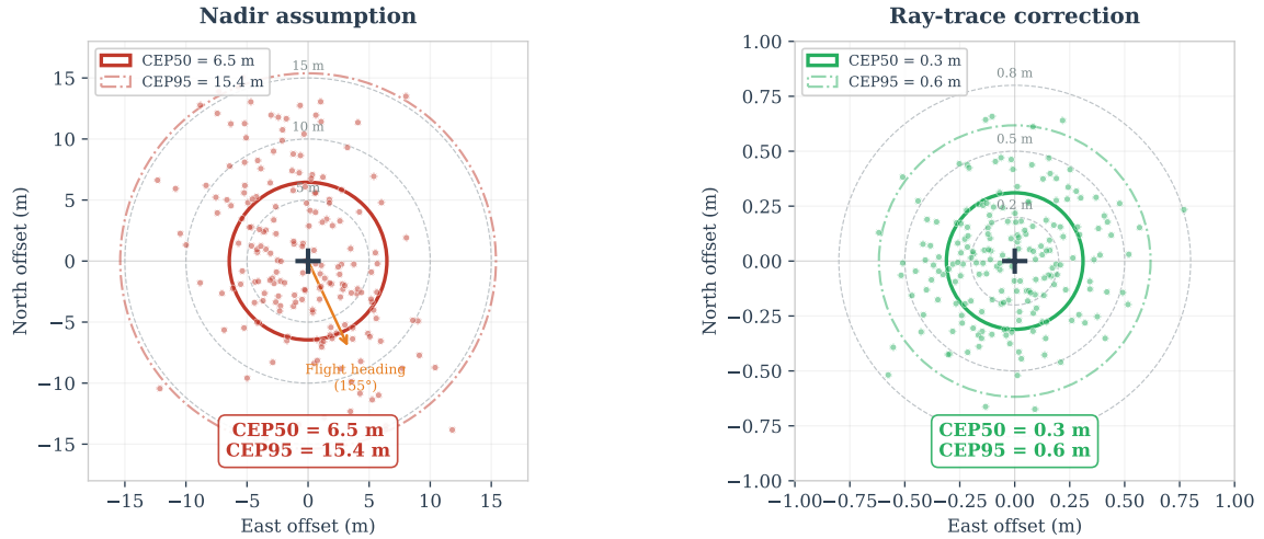
Figure 37: GPS target estimate scatter before and after attitude compensation at 35 m altitude. Without compensation (left), forward-flight pitch introduces a systematic along-track bias of ~6.2 m. With compensation (right), the ray-trace correction reduces the scatter to ~0.3 m, limited by telemetry noise. Data from the 1440-test verification sweep described above.
