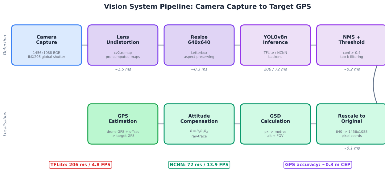
Figure 25: End-to-end vision pipeline: from raw CSI-2 capture through lens undistortion, resize, TFLite inference, confidence filtering, and GPS coordinate projection. Stage timings are measured on the Raspberry Pi 5; total latency is 208 ms per frame (Table 43).
