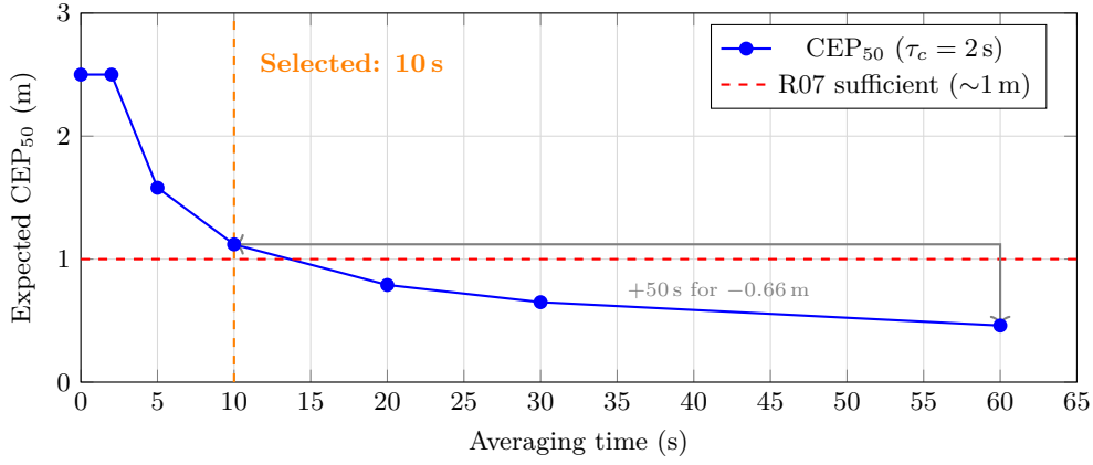
Figure 39: CEP 50 vs. GPS averaging time during stationary hover. The 1/\sqrt{T} convergence means that doubling the averaging time only improves accuracy by \sim 29\% . The 10 s operating point (orange) achieves sub-1.2 m CEP while adding minimal mission time.
