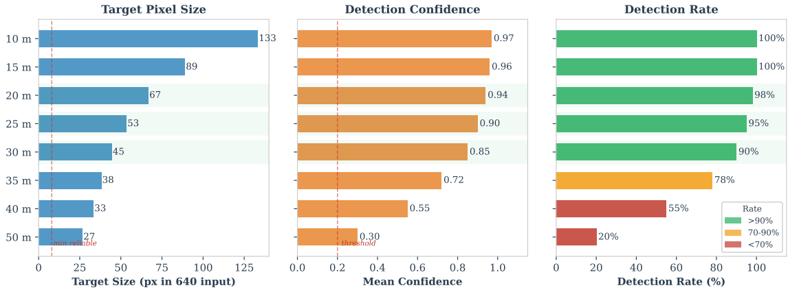
Figure 27: Detection performance as a function of altitude for the YOLOv8n custom model against a 1.8 m mannequin target. The table combines predicted pixel sizes from the thin-lens model with empirically observed confidence and detection rates from video replay analysis.
