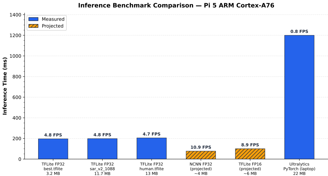
Figure 24: Inference backend comparison on Raspberry Pi 5 for YOLOv8n (640 × 640 input). TFLite with XNNPACK provides the measured production baseline at 4.8FPS; NCNN and FP16 projections indicate viable paths to real-time performance.
