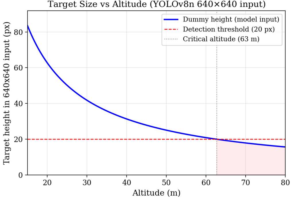
Figure 30: Target height in the 640 \times 640 model input as a function of altitude. The red dashed line marks the 20 px detection threshold; the shaded region indicates unreliable detection.
