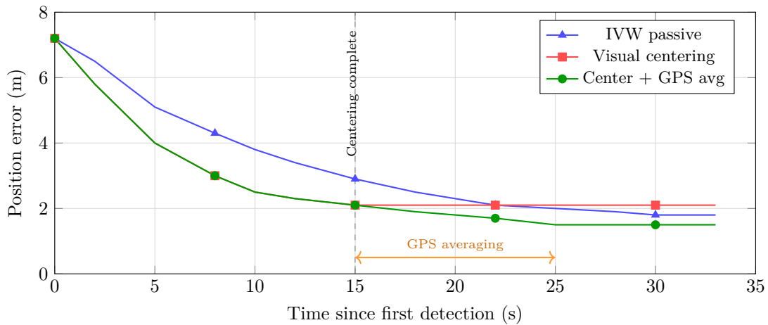
Figure 34: Convergence of position error over time for the three best estimation strategies. All three begin with the same initial flyover estimate (~7 m). Visual centering converges rapidly to 2.1 m (GPS noise floor for single fixes) by t = 15 s. GPS averaging during the subsequent 10 s hold reduces the error further to 1.5 m. IVW converges more slowly because it relies on accumulating many flyover observations rather than actively centering.
