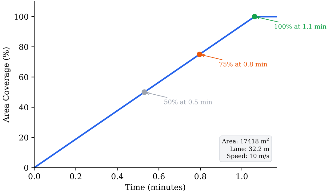
Figure 6: Area coverage progression over time for the boustrophedon search pattern at 35 m altitude. The near-linear increase confirms systematic, gap-free coverage.
