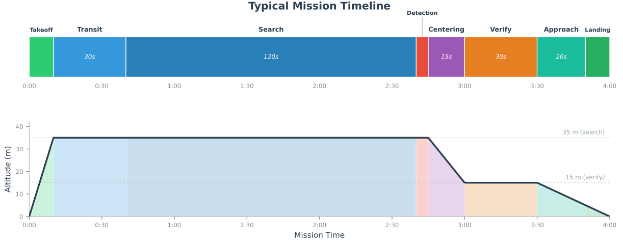
Figure 10: Mission timeline showing state transitions during a simulated end-to-end SAR mission. The horizontal axis represents elapsed time; coloured blocks indicate active states.
