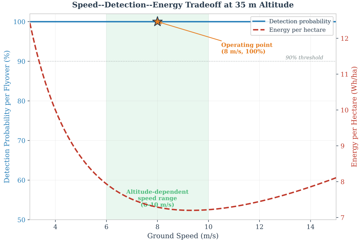
Figure 25: Speed–detection–energy trade-off at 35 m altitude. Detection probability remains above 99.6% across all speeds; the binding constraint is energy consumption and NFZ margin rather than detection reliability.
