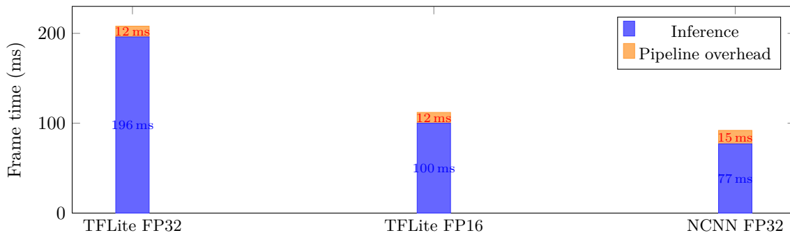
Figure 21: Frame time decomposition: inference vs. pipeline overhead for each backend. As raw inference latency decreases, overhead transitions from negligible (5.8% for TFLite FP32) to significant (16.3% for NCNN).
