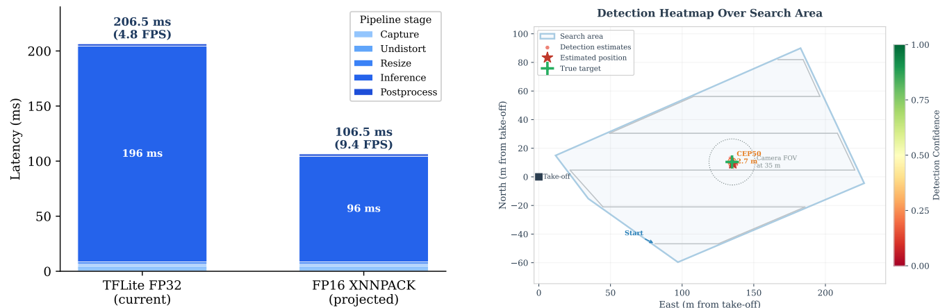
(a) Per-frame latency breakdown: capture, undistortion, resize, inference, and postprocessing. (b) Spatial detection heatmap showing detection density across the survey area during simulated search.
