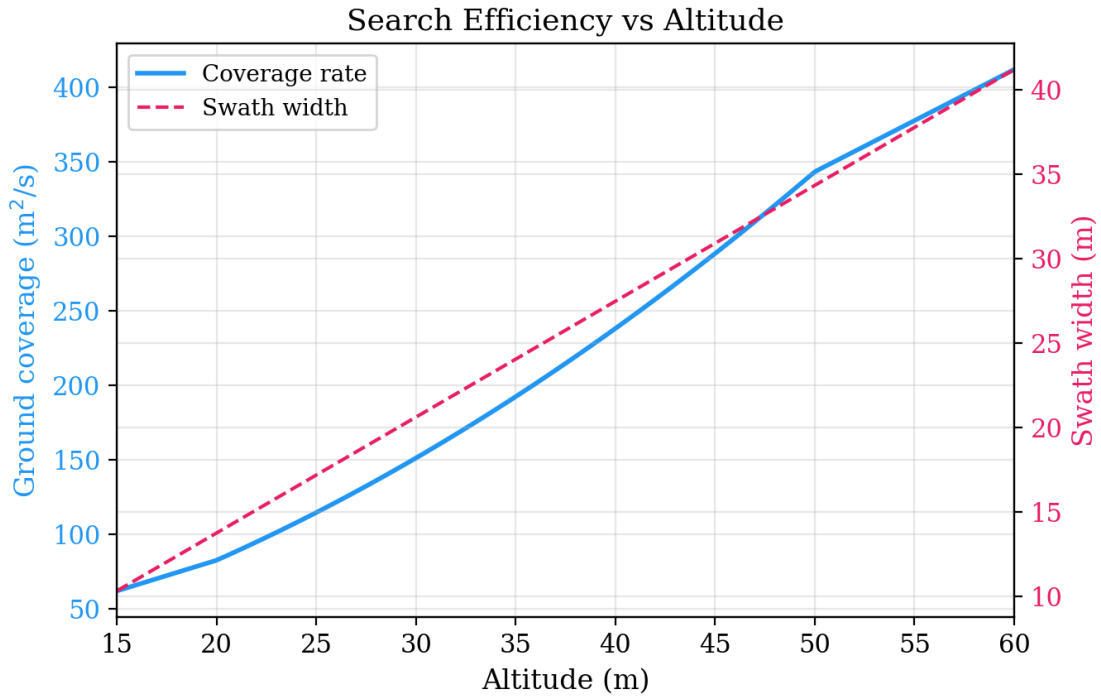
Figure 33: Search efficiency vs. altitude. The solid blue line shows coverage rate ( \text{m}^2/\text{s} ); the dashed pink line shows swath width. Higher altitude improves efficiency at the cost of reduced target pixel size.
