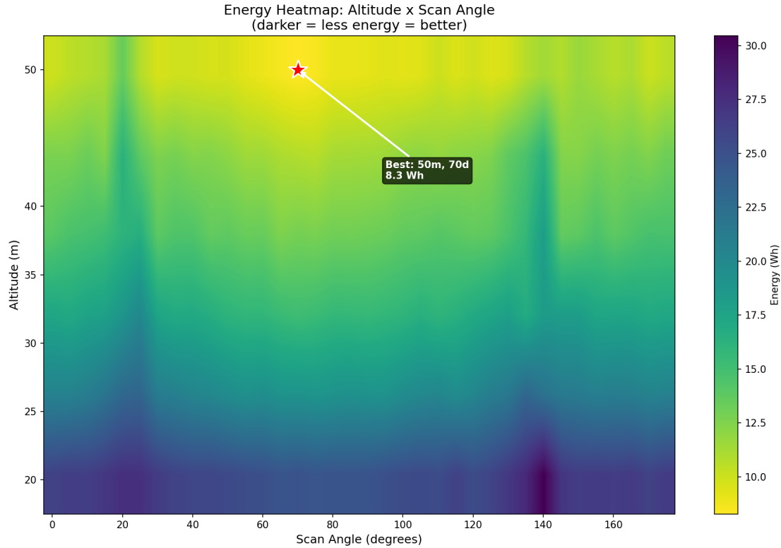
Figure 26: Energy heatmap across 216 altitude–angle configurations. The colour scale represents total energy consumption including NFZ slowdown penalties. A clear valley of low-energy configurations runs through the 65° to 75° scan angle band at all altitudes, corresponding to alignment with the polygon’s longest edge. The red star marks the global energy minimum at 50 m altitude and 70° scan angle.
