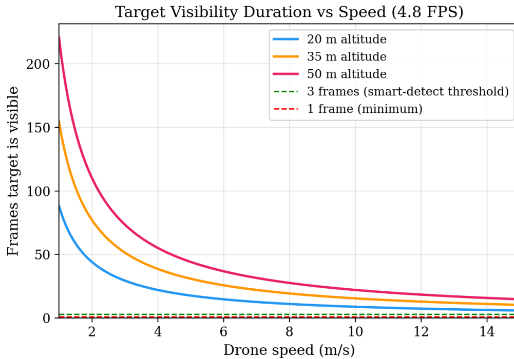
Figure 32: Frames the target remains visible vs. drone speed at three altitudes (4.8 FPS). The green and red dashed lines mark the 3-frame smart-detect threshold and 1-frame minimum, respectively.
