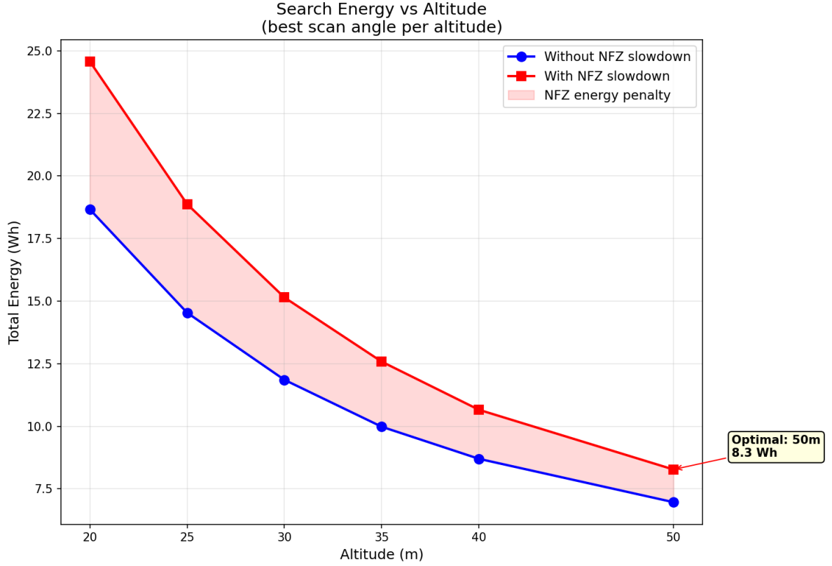
Figure 27: Total search energy versus altitude at the optimal scan angle, with and without NFZ slowdown. The NFZ penalty is most pronounced at 20 m, where several scan lines pass through the slow zone near the SSSI boundary. The shaded region quantifies the additional hover energy incurred by the speed ramp.
