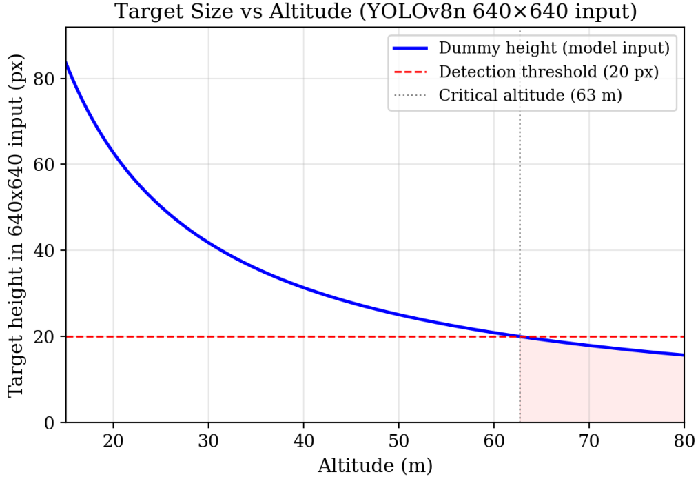
Figure 30: Target height in the 640×640 model input as a function of altitude. The red dashed line marks the 20 px detection threshold; the shaded region indicates unreliable detection.
