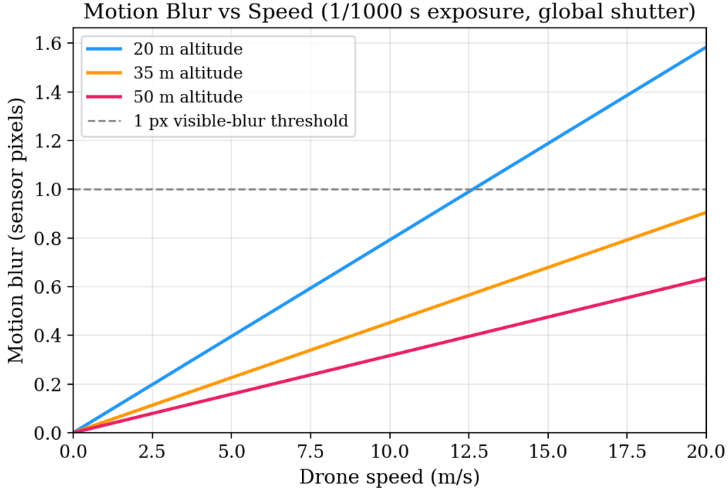
Figure 31: Motion blur vs. drone speed at three altitudes (1/1000 s exposure, global shutter). The grey dashed line marks the 1 px visible-blur threshold.
