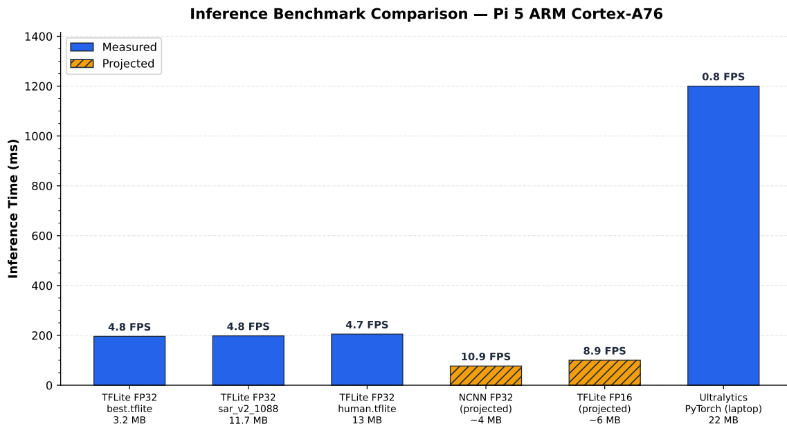
Figure 18: Inference backend comparison on Raspberry Pi 5 for YOLOv8n ( 640 \times 640 input). TFLite with XNNPACK provides the measured production baseline at 4.8FPS; NCNN and FP16 projections indicate viable paths to real-time performance.
