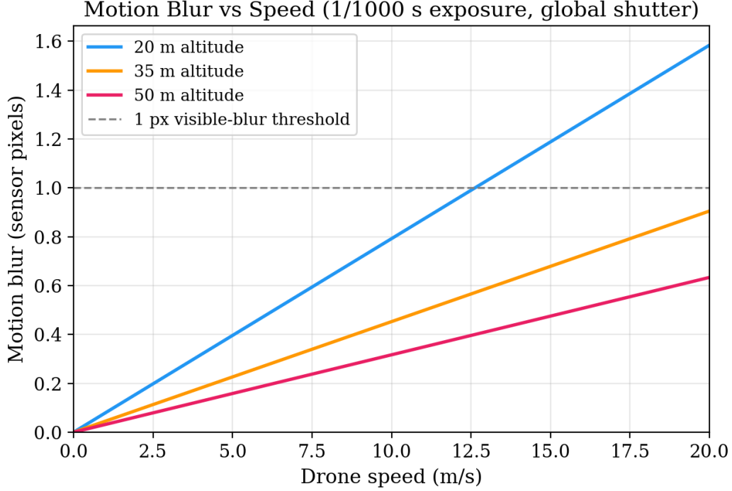
Figure 76: Motion blur vs. drone speed at three altitudes (1/1000 s exposure, global shutter). The grey dashed line marks the 1 px visible-blur threshold.
