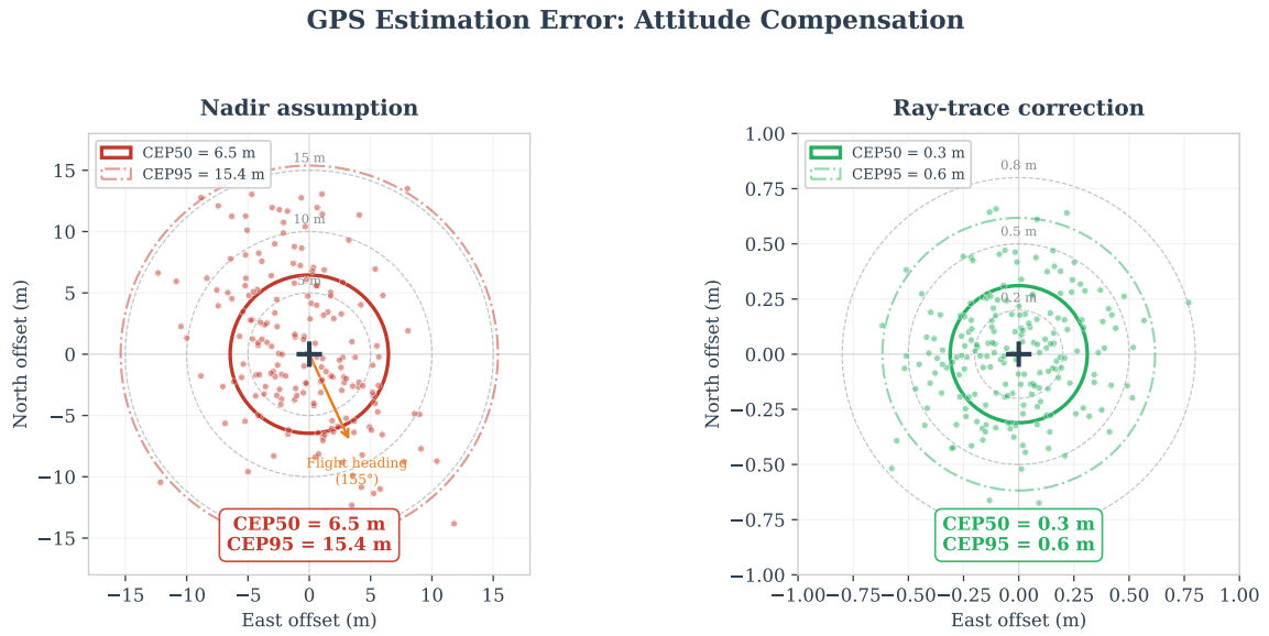
Figure 29: GPS target estimate scatter before and after attitude compensation at 35 m altitude. Without compensation (left), forward-flight pitch introduces a systematic along-track bias of \sim 6.2 m. With compensation (right), the ray-trace correction reduces the scatter to \sim 0.3 m, limited by telemetry noise. Data from the 1440-test verification sweep described above.
