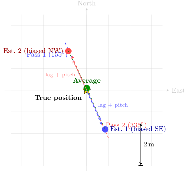
Figure 39: Multi-pass bias cancellation. Pass 1 (heading 155^\circ , blue) biases the GPS estimate south-east; Pass 2 (heading 335^\circ , red) biases it north-west by the same magnitude. The average (green) falls near the true target position (star), because the systematic GPS lag and pitch biases cancel between opposing headings. Only random GPS receiver noise remains.
