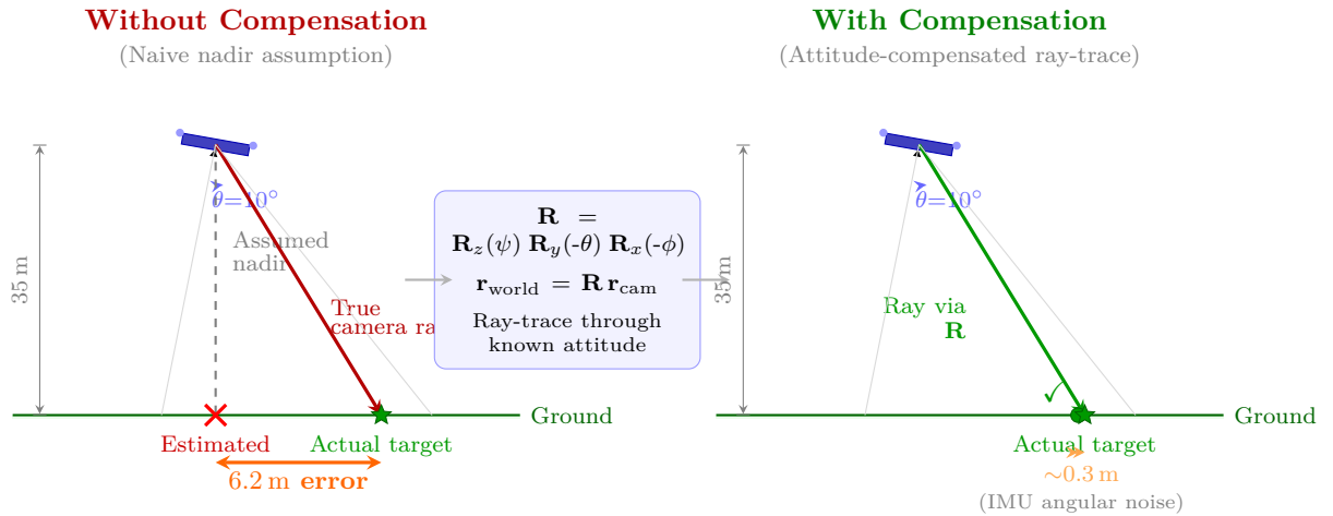
Figure 28: GPS estimation with and without attitude compensation at 10^\circ pitch and 35 m altitude. Left: the naive nadir assumption projects the detection straight below the drone, producing a 6.2 m systematic error equal to h \tan \theta . Right: the attitude-compensated estimator ray-traces the detection pixel through the full rotation matrix \mathbf{R} constructed from real-time telemetry, recovering the true ground position; the residual \sim 0.3 m error is due to IMU angular noise only ( \pm 0.5^\circ ).
