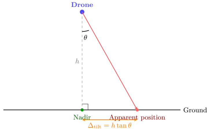
Figure 27: Roll/pitch geometry. A drone tilted at angle \theta from vertical projects the optical axis forward by \Delta_{\text{tilt}} = h \tan \theta . At 35 m and \theta = 10^\circ , this displacement is 6.2 m—larger than GPS receiver noise. During hover ( \theta < 1^\circ ), the displacement is < 0.6 \text{ m} .
