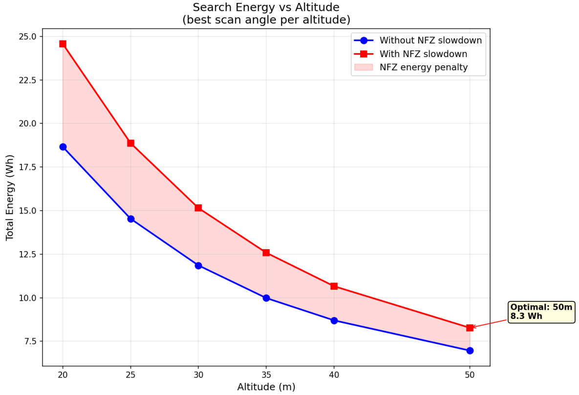
Figure 48: Total search energy versus altitude at the optimal scan angle, with and without NFZ slowdown. The NFZ penalty is most pronounced at 20 m, where several scan lines pass through the slow zone near the SSSI boundary. The shaded region quantifies the additional hover energy incurred by the speed ramp.
