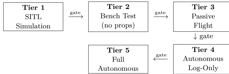
Figure 40: Tier progression. Each arrow represents a gate: the downstream tier is blocked until all upstream tests pass.
