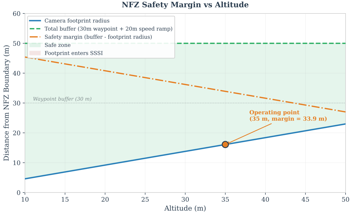
Figure 45: NFZ margin analysis as a function of altitude. The camera footprint radius grows linearly with altitude, but the implemented 50 m total margin maintains a comfortable surplus at all operational altitudes.
