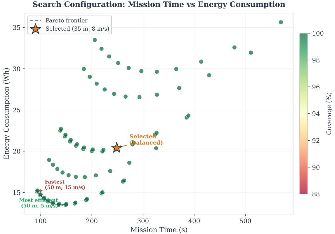
Figure 43: Energy efficiency across the 216-configuration parameter sweep. Lower-energy configurations cluster at high altitude and optimal scan angle; the selected operating point ( 35 \text{ m} , 70^\circ , 8 \text{ m s}^{-1} ) trades minimal energy for reliable detection.
