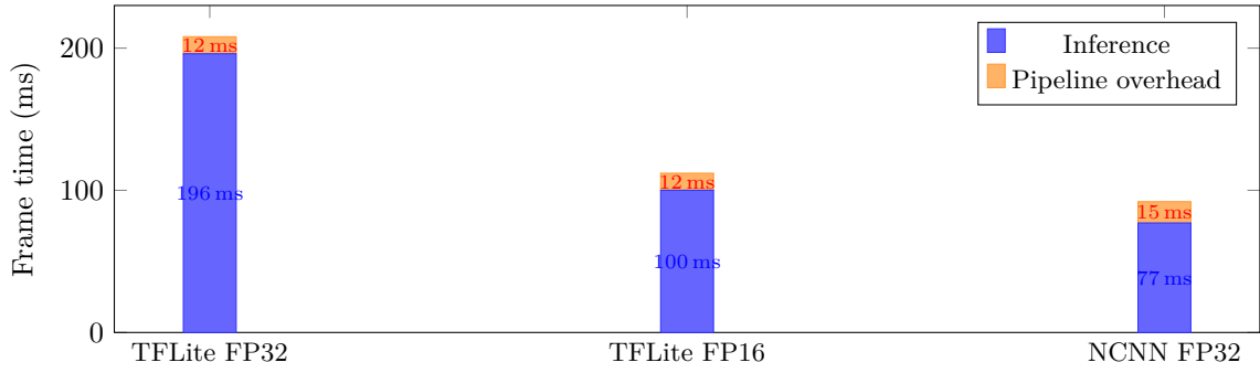
Figure 26: Frame time decomposition: inference vs. pipeline overhead for each backend. As raw inference latency decreases, overhead transitions from negligible (5.8% for TFLite FP32) to significant (16.3% for NCNN).
