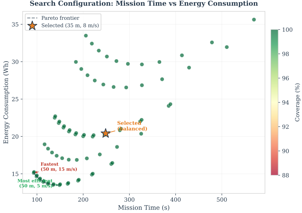
Figure 49: Energy efficiency across the operating range. The search phase consumes only 10.9% of battery capacity at the selected operating point, leaving ample margin for transit, descent phases, and RTL.
