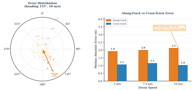
(b) Directional error distribution showing heading-aligned elongation from GPS timing lag.
