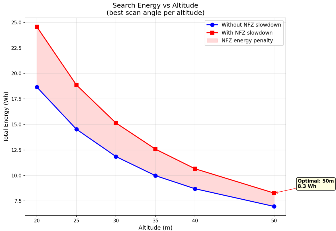
Figure 32: Total search energy versus altitude at the optimal scan angle, with and without NFZ slowdown. The NFZ penalty is most pronounced at 20 m, where several scan lines pass through the slow zone near the SSSI boundary. The shaded region quantifies the additional hover energy incurred by the speed ramp.
