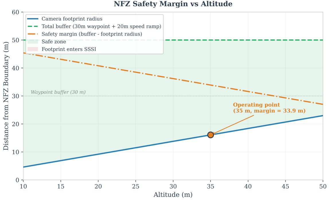
Figure 29: NFZ margin analysis as a function of altitude. The camera footprint radius grows linearly with altitude, but the implemented 50 m total margin maintains a comfortable surplus at all operational altitudes.
