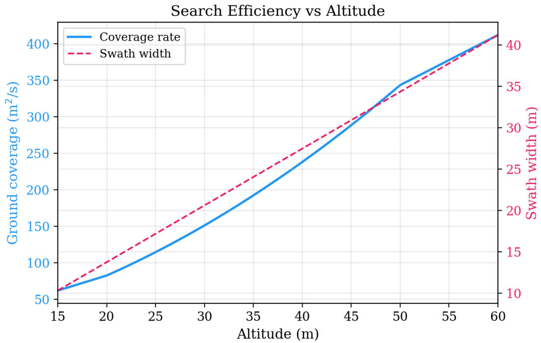
Figure 62: Search efficiency vs. altitude. The solid blue line shows coverage rate ( \text{m}^2/\text{s} ); the dashed pink line shows swath width. Higher altitude improves efficiency at the cost of reduced target pixel size.
