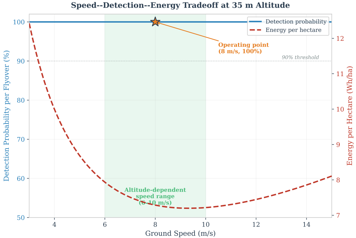
Figure 30: Speed–detection–energy trade-off at 35 m altitude. Detection probability remains above 99.6% across all speeds; the binding constraint is energy consumption and NFZ margin rather than detection reliability.
