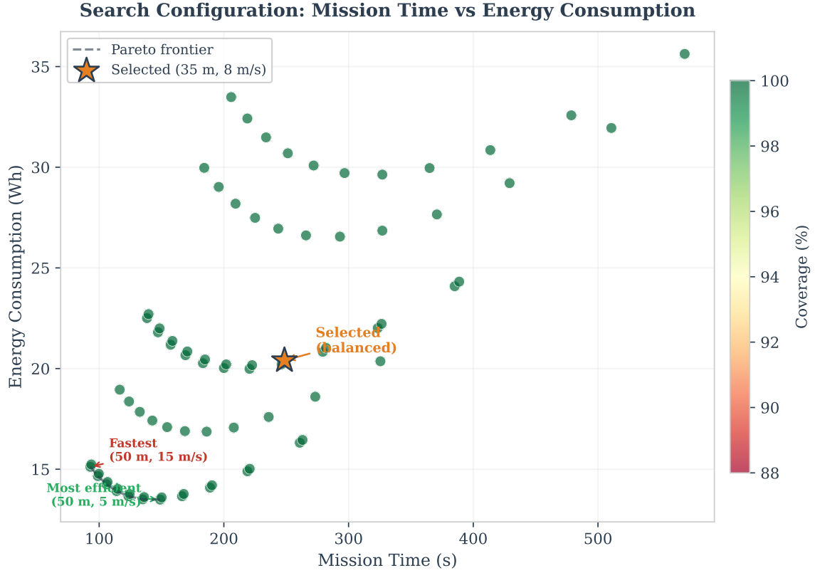
Figure 27: Energy efficiency across the 216-configuration parameter sweep. Lower-energy configurations cluster at high altitude and optimal scan angle; the selected operating point (35 m, 70°, 8 m s -1 ) trades minimal energy for reliable detection.
