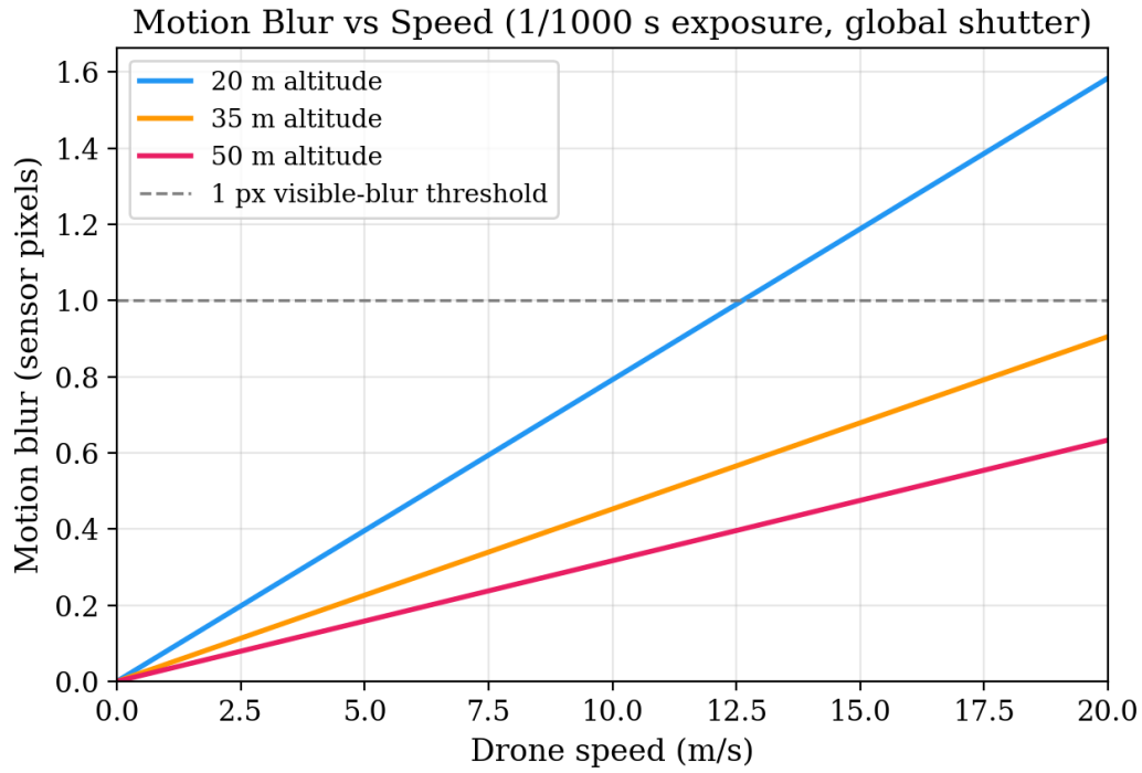
Figure 60: Motion blur vs. drone speed at three altitudes (1/1000 s exposure, global shutter). The grey dashed line marks the 1 px visible-blur threshold.
