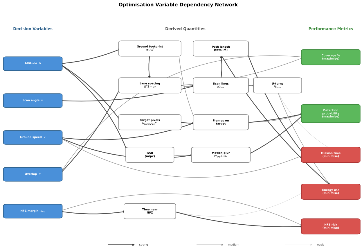
Figure 52: Optimisation variable dependency network. Decision variables (blue) cascade through derived quantities (white) to performance metrics (green/red). Arrow thickness indicates influence strength.
