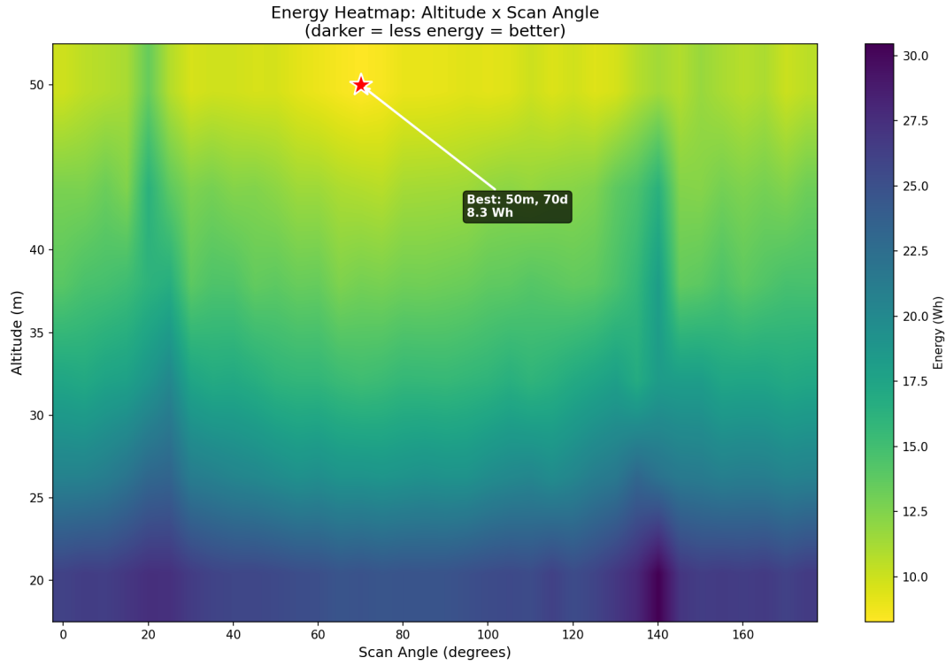
Figure 40: Energy heatmap across 216 altitude–angle configurations. A clear low-energy valley runs through 65\text{--}75^\circ at all altitudes, corresponding to longest-edge alignment. The red star marks the global energy minimum (50 m, 70^\circ ). The selected point (35 m, 70^\circ ) trades 4.4 Wh of energy for a 44% increase in target pixel extent.
