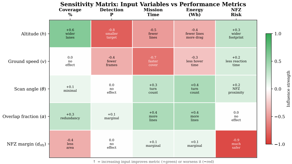
Figure 53: Sensitivity matrix showing the influence of each input parameter on every derived quantity. Darker cells indicate stronger coupling, revealing which measurements most critically affect mission performance.
