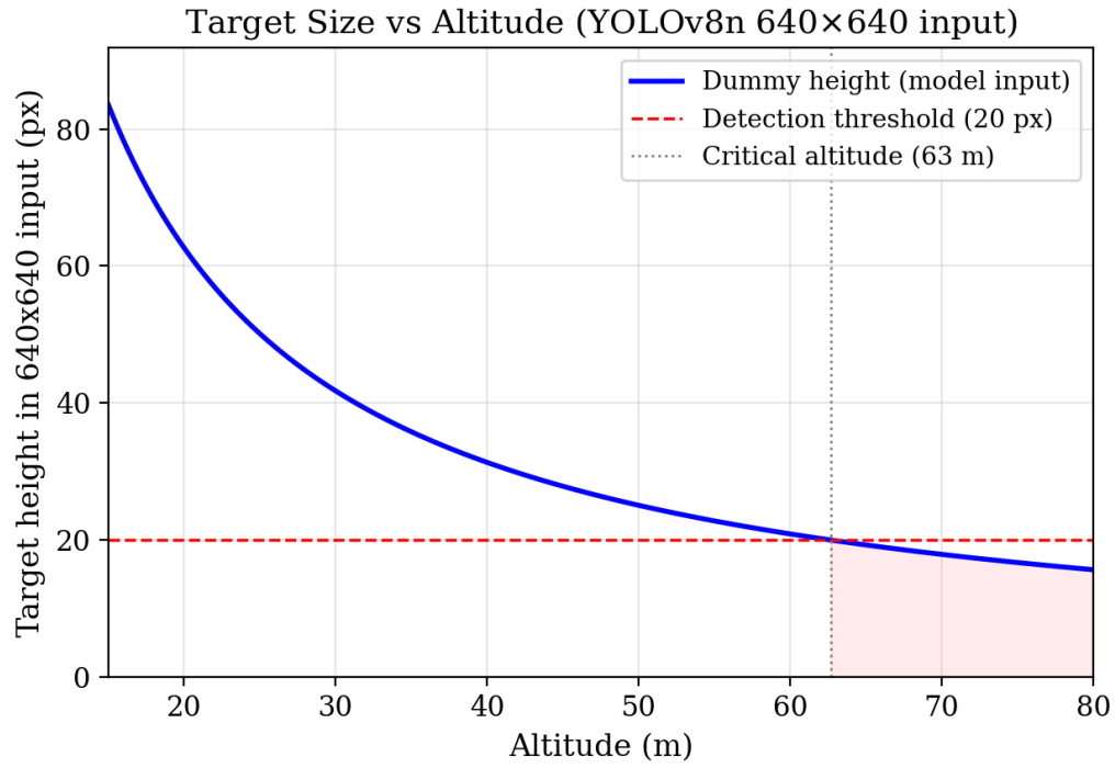
Figure 41: Target height in the 640×640 model input as a function of altitude. The red dashed line marks the 20 px detection threshold; the shaded region indicates unreliable detection.
