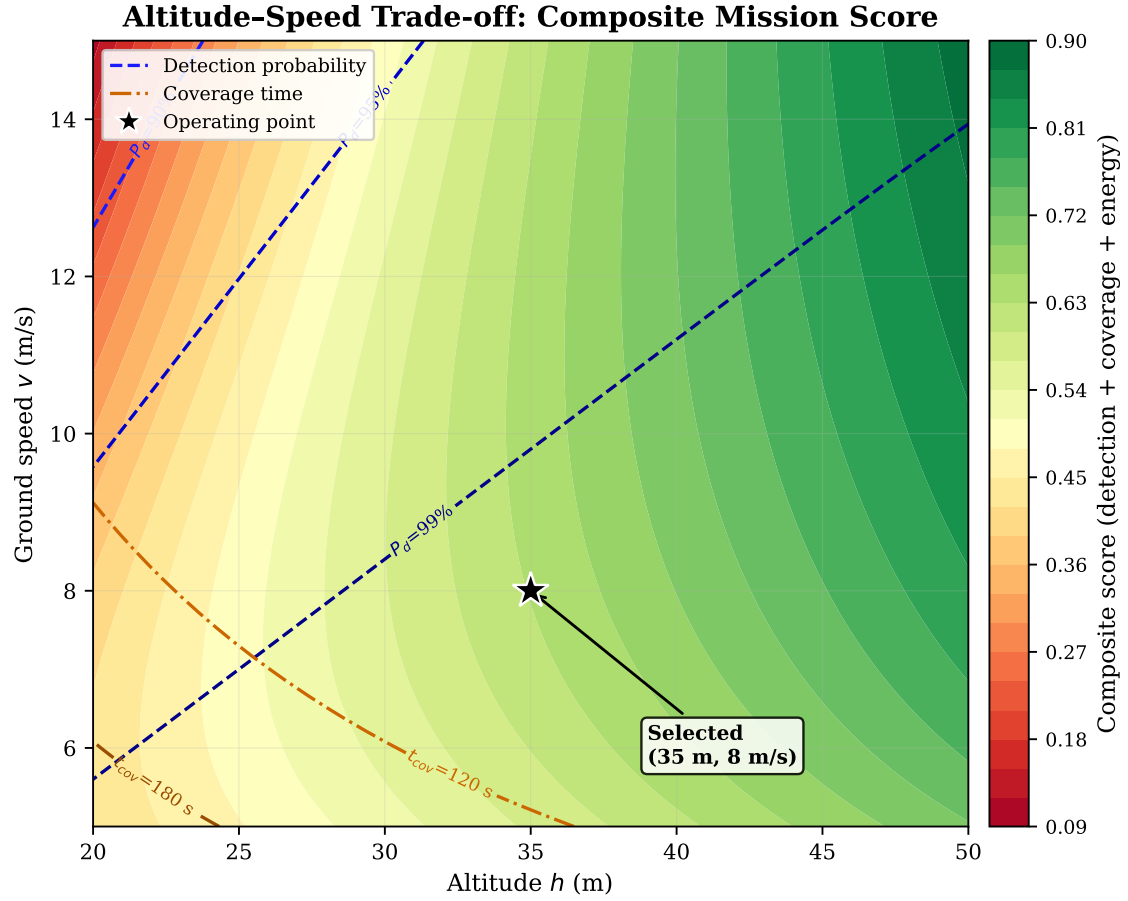
Figure 40: Altitude–speed trade-off space. Colour shows composite mission score (40% detection + 35% coverage + 25% energy). Blue contours: detection probability. Orange contours: coverage time. The selected operating point (35 m, 8 m/s) sits above the 95% detection contour in the high-score region.
