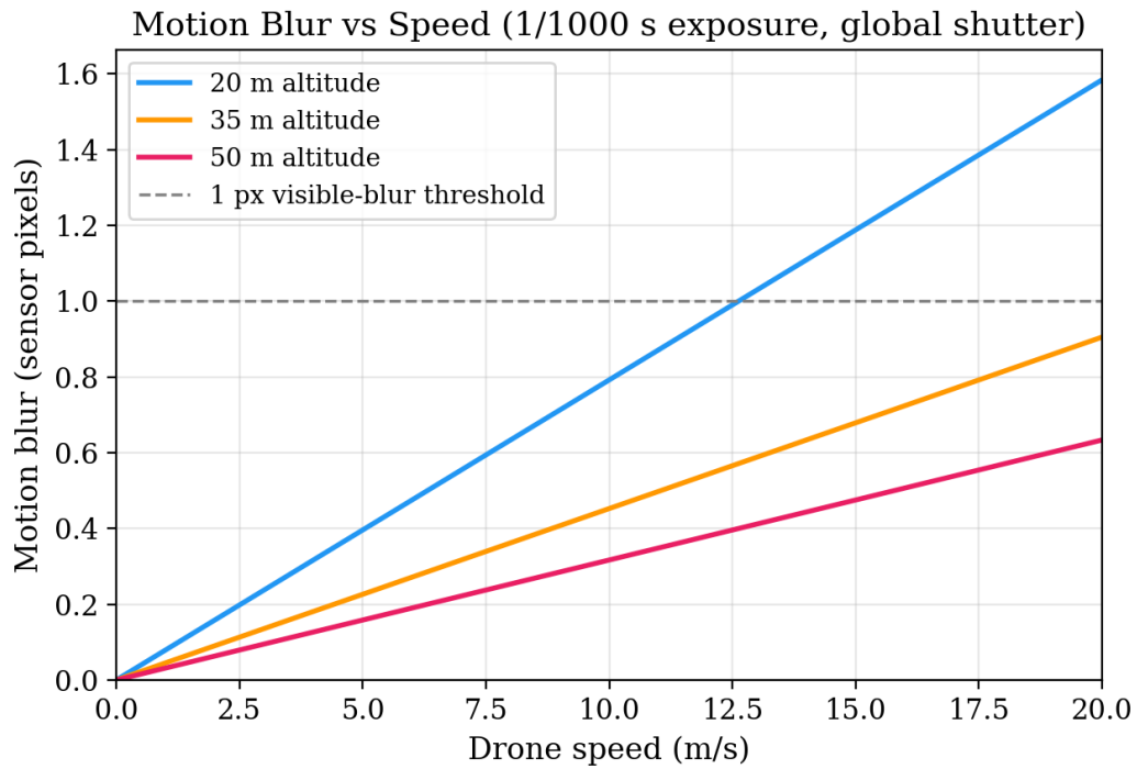
Figure 42: Motion blur vs. drone speed at three altitudes (1/1000 s exposure, global shutter). The grey dashed line marks the 1 px visible-blur threshold.
