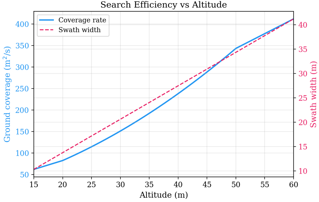
Figure 73: Search efficiency vs. altitude. The solid blue line shows coverage rate ( \text{m}^2/\text{s} ); the dashed pink line shows swath width. Higher altitude improves efficiency at the cost of reduced target pixel size.
