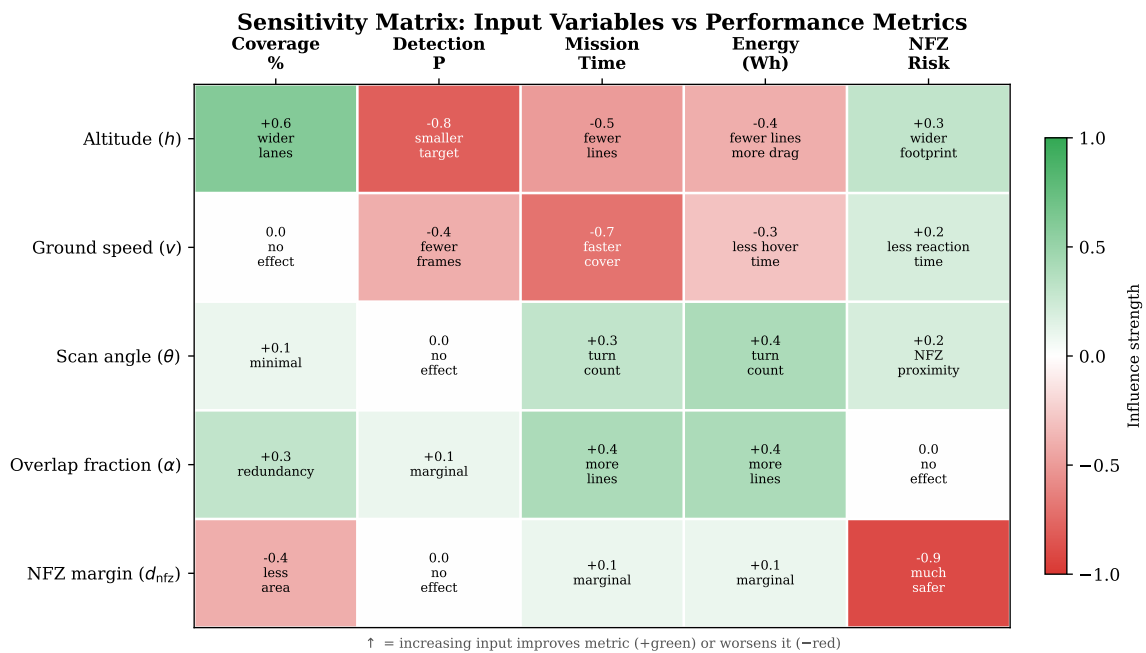
Figure 64: Sensitivity matrix showing the influence of each input parameter on every derived quantity. Darker cells indicate stronger coupling, revealing which measurements most critically affect mission performance.
