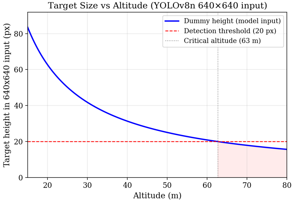
Figure 70: Target height in the 640 \times 640 model input as a function of altitude. The red dashed line marks the 20 px detection threshold; the shaded region indicates unreliable detection.
