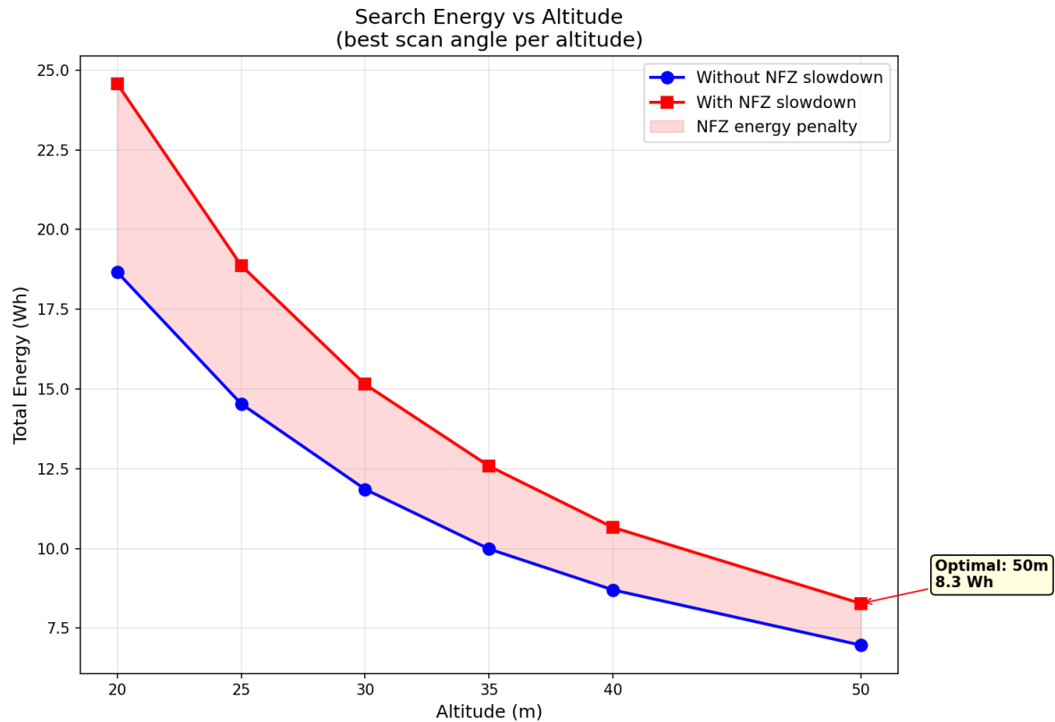
Figure 43: Total search energy versus altitude at the optimal scan angle, with and without NFZ slowdown. The NFZ penalty is most pronounced at 20 m, where several scan lines pass through the slow zone near the SSSI boundary. The shaded region quantifies the additional hover energy incurred by the speed ramp.
