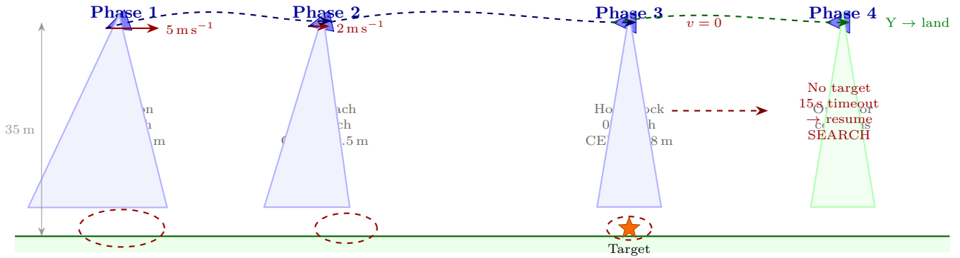
Figure 30: The four-phase progressive refinement trajectory. Phase 1: initial detection at full search speed with tilted camera and tilt-compensated GPS estimate (CEP \approx 3.5 m). Phase 2: continuous approach and deceleration, pitch decreases, estimate improves (CEP \approx 2.5 m). Phase 3: stationary hover with nadir camera, all geometric errors eliminated (CEP \approx 1.8 m); if no target is visible, a 15 s timeout triggers resumption (red dashed branch). Phase 4: operator confirms via ground station; Y triggers offset landing, N resumes search. Error circles are drawn proportional to CEP at each phase.
