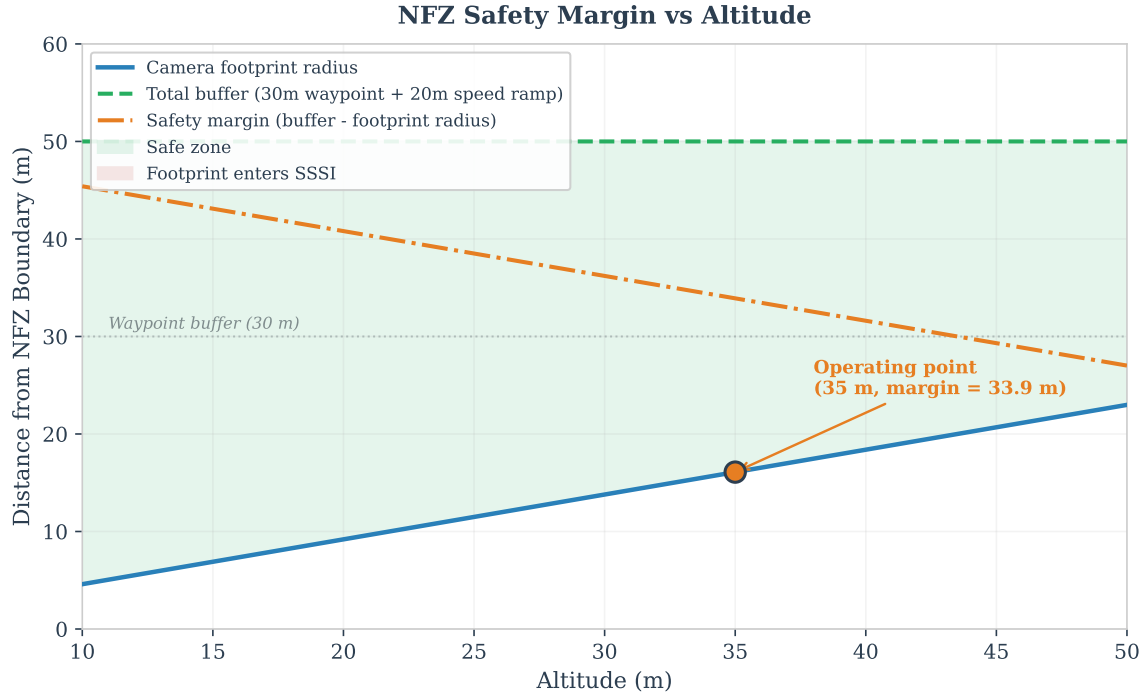
Figure 40: NFZ margin analysis as a function of altitude. The camera footprint radius grows linearly with altitude, but the implemented 50 m total margin maintains a comfortable surplus at all operational altitudes.
