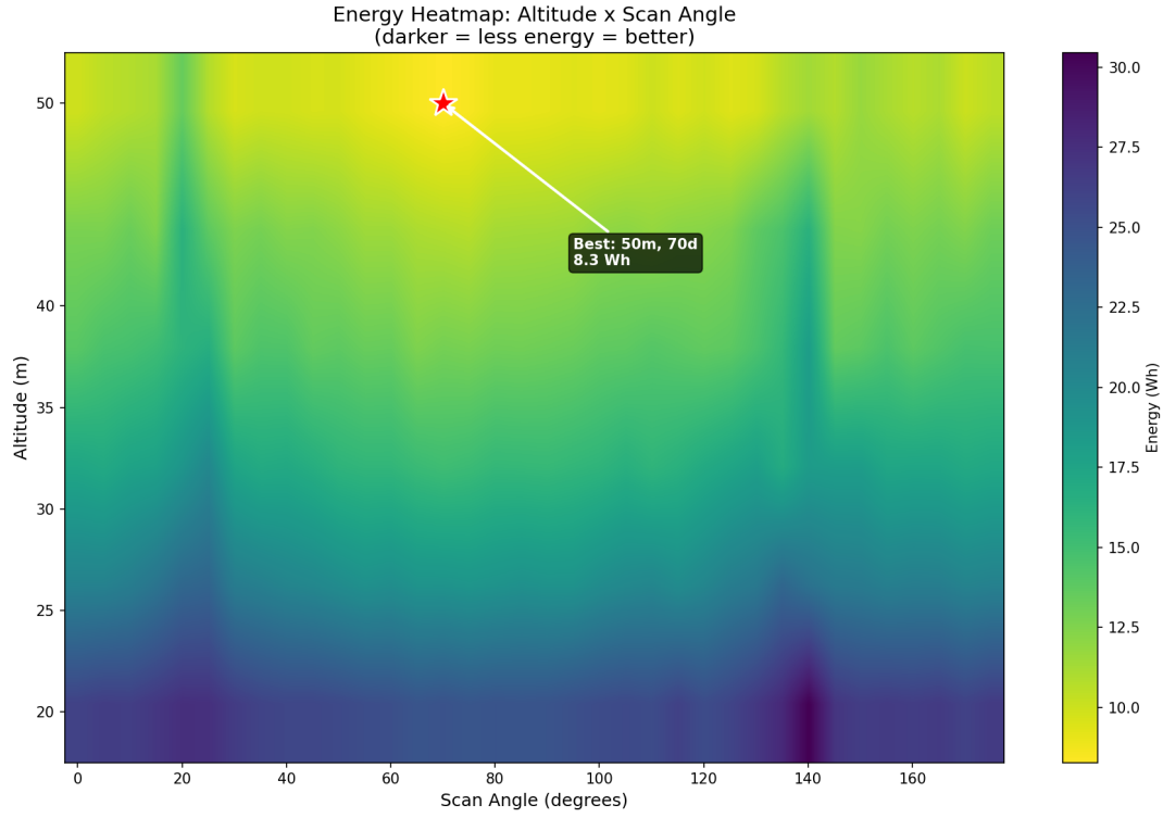
Figure 51: Energy heatmap across 216 altitude–angle configurations. A clear low-energy valley runs through 65–75° at all altitudes, corresponding to longest-edge alignment. The red star marks the global energy minimum (50 m, 70°). The selected point (35 m, 70°) trades 4.4 Wh of energy for a 44% increase in target pixel extent.
