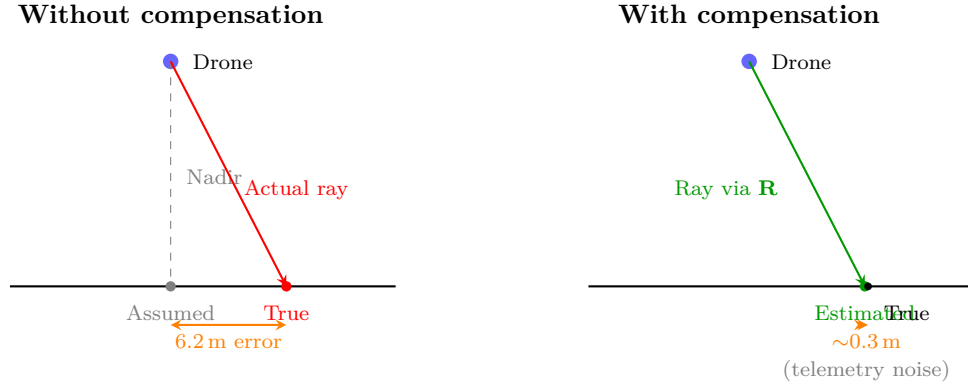
Figure 26: GPS estimation with and without attitude compensation at 10^\circ pitch and 35 m altitude. Left: nadir assumption projects the detection directly below the drone, producing 6.2 m error. Right: ray-tracing through the rotation matrix \mathbf{R} recovers the true ground position; the residual \sim 0.3 m error is due to IMU angular noise only.
