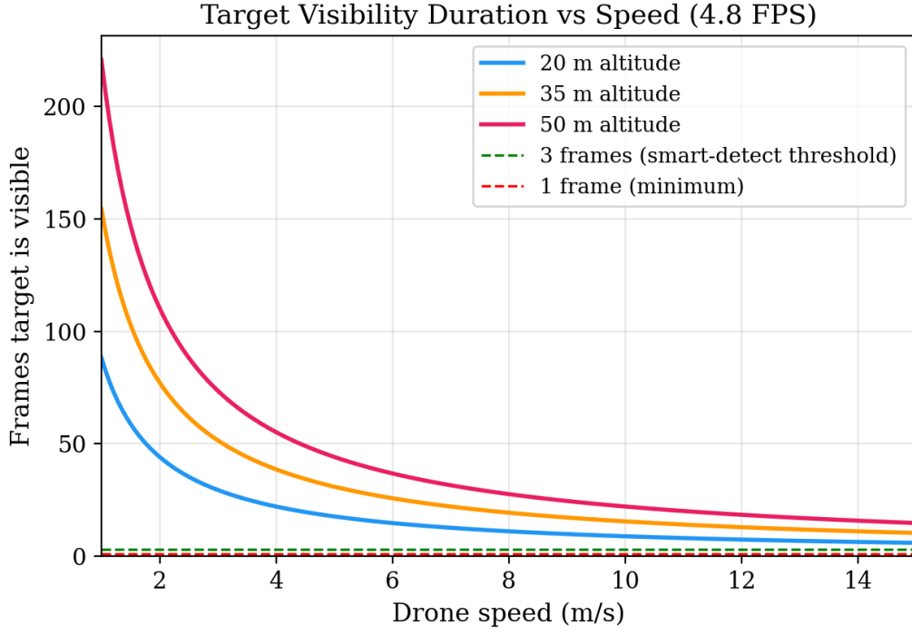
Figure 72: Frames the target remains visible vs. drone speed at three altitudes (4.8 FPS). The green and red dashed lines mark the 3-frame smart-detect threshold and 1-frame minimum, respectively.
