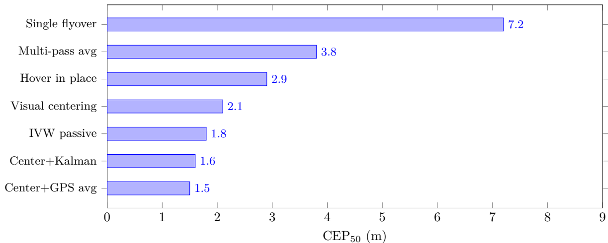
Figure 32: \text{CEP}_{50} comparison across seven GPS estimation strategies (lower is better). The centering + GPS averaging approach achieves 1.5 m—a 4.8\times improvement over a single flyover estimate. Error bars omitted for clarity; inter-trial variation was <0.3 \text{ m} for all strategies except “single flyover” ( \pm 1.1 \text{ m} ).
