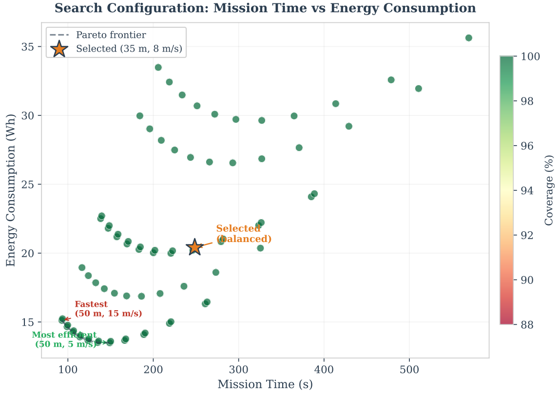
Figure 38: Energy efficiency across the 216-configuration parameter sweep. Lower-energy configurations cluster at high altitude and optimal scan angle; the selected operating point (35 m, 70°, 8 m s -1 ) trades minimal energy for reliable detection.
