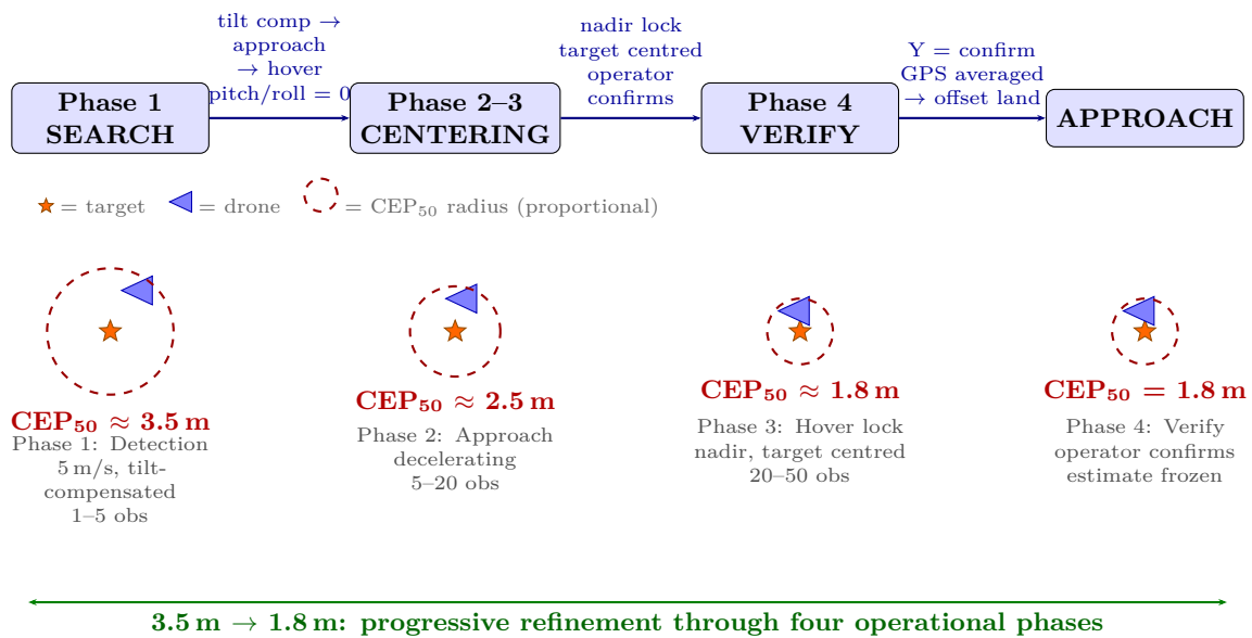
Figure 32: Target GPS estimate accuracy progression through the four-phase detection-to-landing flow. Circle radii are proportional to CEP_{50} at each phase. Tilt compensation in Phase 1 reduces the initial estimate from \sim 7 m (uncompensated) to \sim 3.5 m. The combination of continuous approach refinement (Phase 2), hover lock with nadir camera (Phase 3), operator verification with GPS averaging (Phase 4), and spatial deduplication of false positives transforms the initial estimate into a \sim 1.8 m final position—a \sim 2\times improvement through operational procedure alone.
