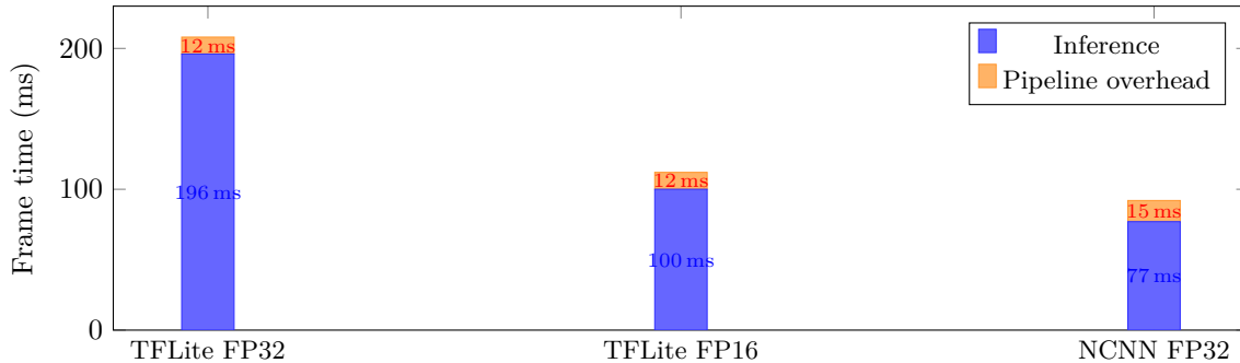
Figure 42: Frame time decomposition: inference vs. pipeline overhead for each backend. As raw inference latency decreases, overhead transitions from negligible (5.8% for TFLite FP32) to significant (16.3% for NCNN).
