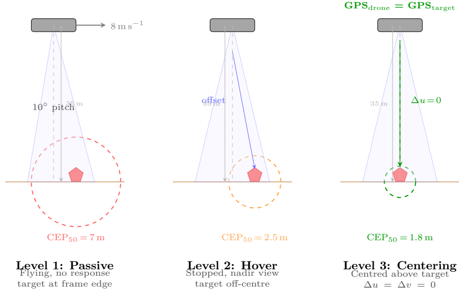
Figure 30: Side-by-side comparison of the three estimation levels. Dashed circles represent the \text{CEP}_{50} error radius around the true target position (star). Level 1 (passive): the drone is pitched forward and moving, placing the target at the frame edge with the largest error circle. Level 2 (hover): the drone is stationary and nadir-pointing, but the target remains off-centre, requiring the full projection pipeline. Level 3 (centering): the drone has manoeuvred directly above the target, driving the pixel offset to zero and collapsing the error to GPS receiver noise only.
