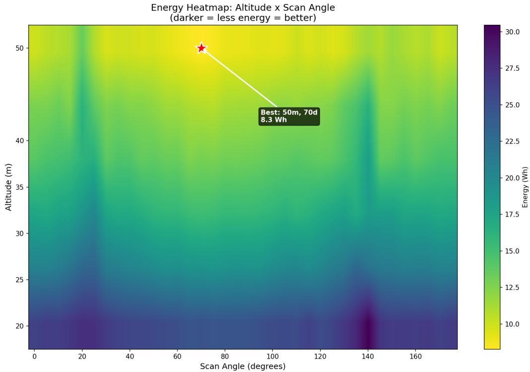
Figure 52: Energy heatmap across 216 altitude–angle configurations. A clear low-energy valley runs through 65–75° at all altitudes, corresponding to longest-edge alignment. The red star marks the global energy minimum (50 m, 70°). The selected point (35 m, 70°) trades 4.4 Wh of energy for a 44% increase in target pixel extent.
