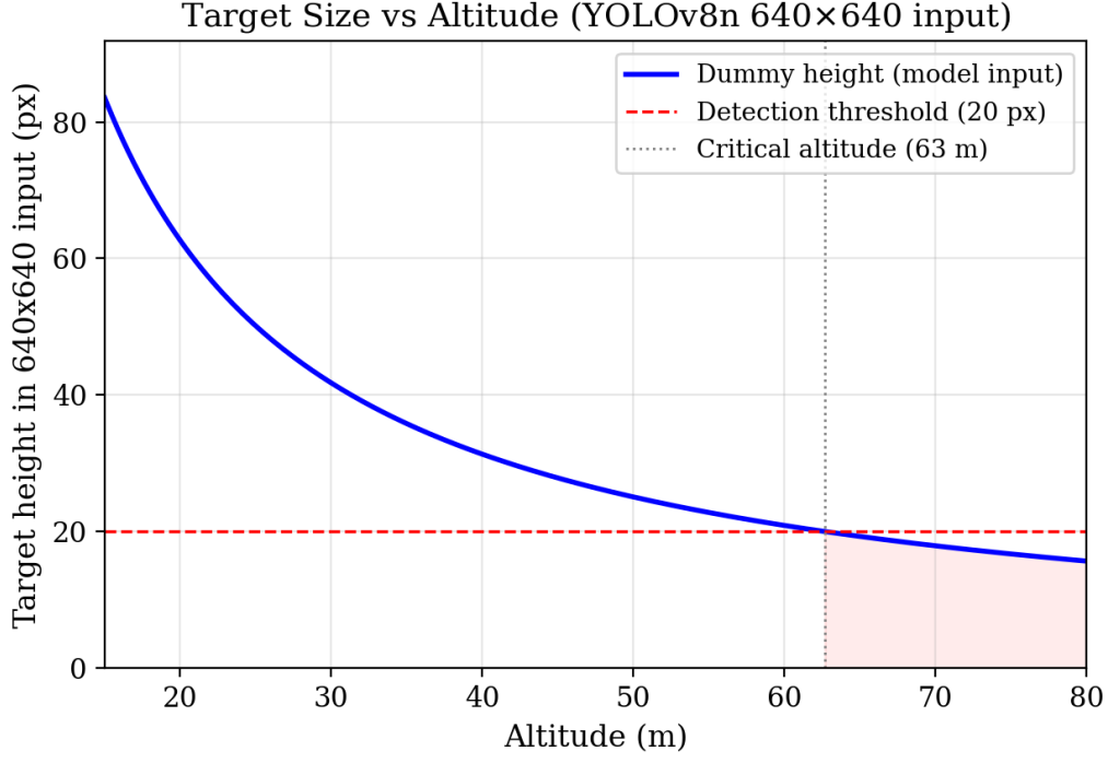
Figure 31: Target height in the 640×640 model input as a function of altitude. The red dashed line marks the 20 px detection threshold; the shaded region indicates unreliable detection.
