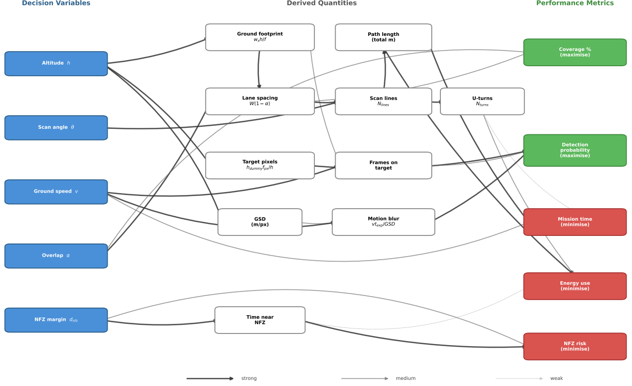
Figure 30: Optimisation variable dependency network. Decision variables (blue) cascade through derived quantities (white) to performance metrics (green/red). Arrow thickness indicates influence strength.
