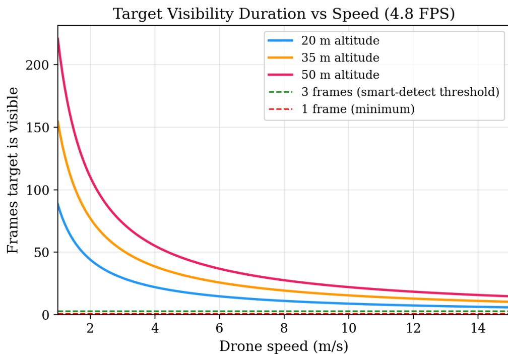
Figure 33: Frames the target remains visible vs. drone speed at three altitudes (4.8 FPS). The green and red dashed lines mark the 3-frame smart-detect threshold and 1-frame minimum, respectively.
