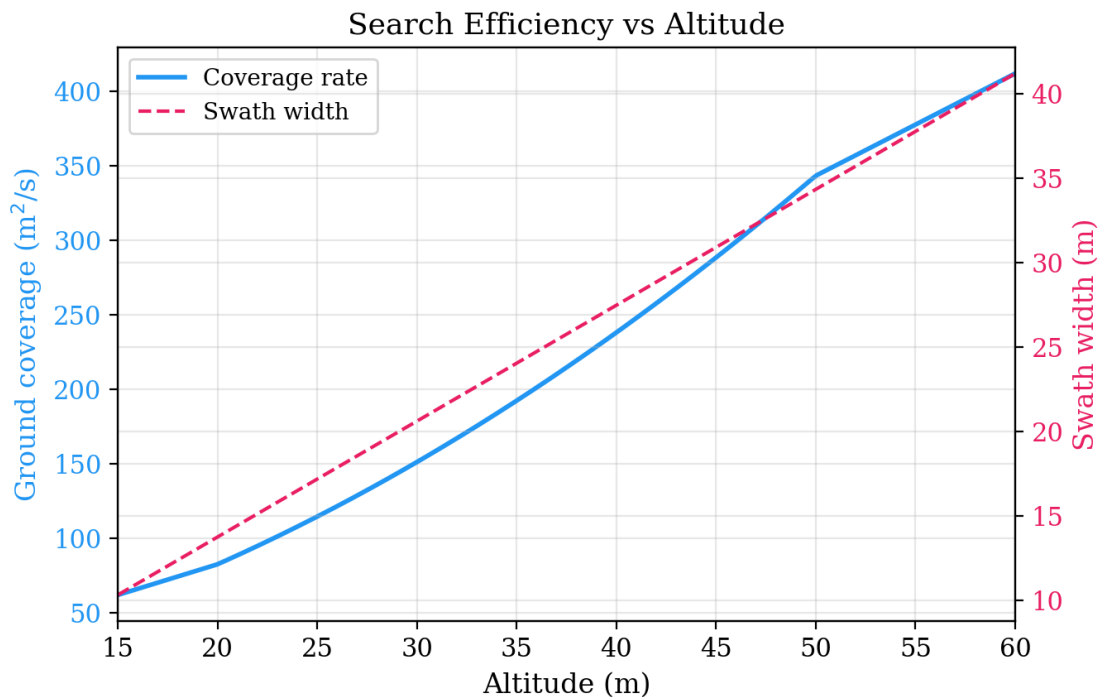
Figure 34: Search efficiency vs. altitude. The solid blue line shows coverage rate ( \text{m}^2/\text{s} ); the dashed pink line shows swath width. Higher altitude improves efficiency at the cost of reduced target pixel size.
