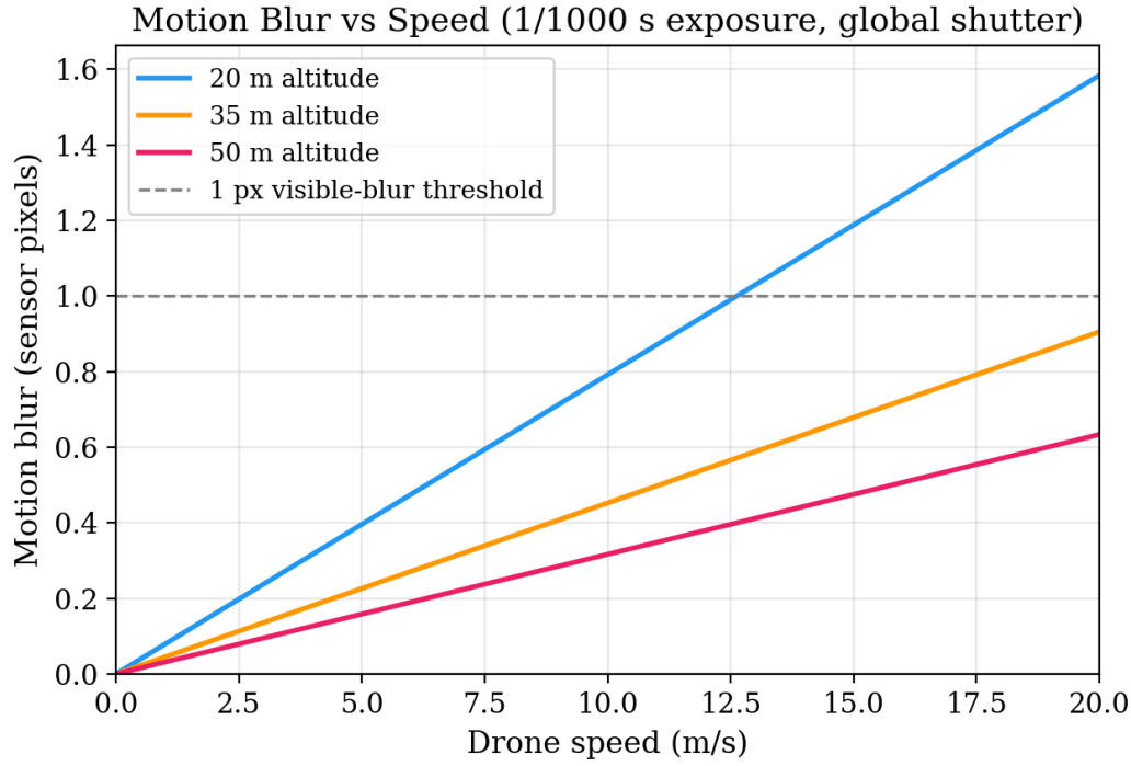
Figure 32: Motion blur vs. drone speed at three altitudes (1/1000 s exposure, global shutter). The grey dashed line marks the 1 px visible-blur threshold.
