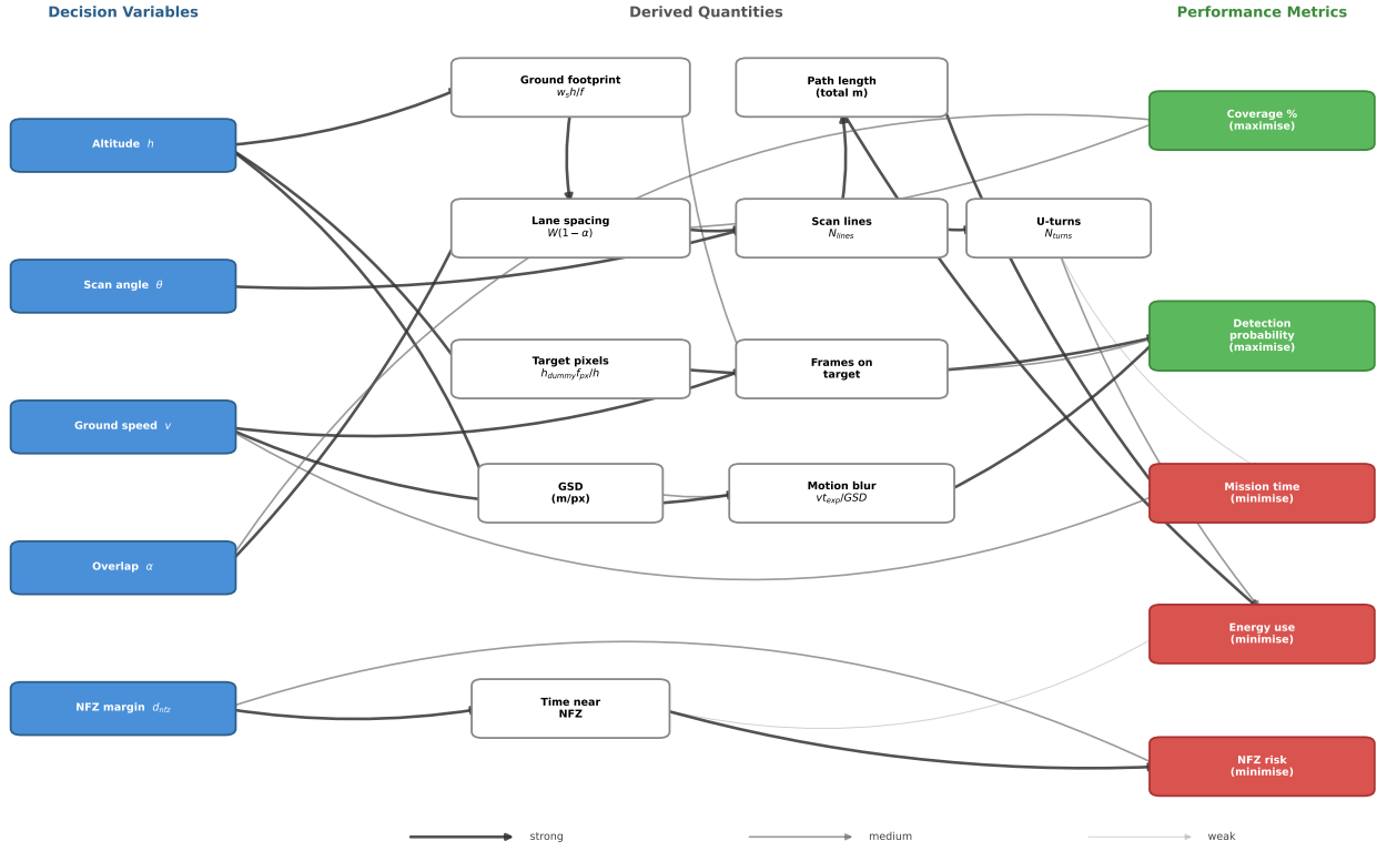
Figure 36: Optimisation variable dependency network. Decision variables (blue) cascade through derived quantities (white) to performance metrics (green/red). Arrow thickness indicates influence strength.
