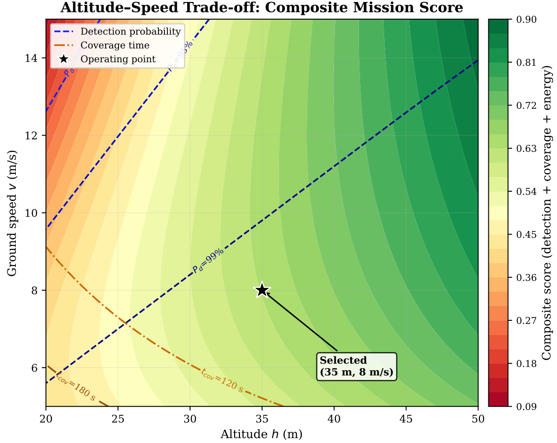
Figure 40: Altitude-speed trade-off space. Colour shows composite mission score (40% detection + 35% coverage + 25% energy). Blue contours: detection probability. Orange contours: coverage time. The selected operating point (35 m, 8 m/s) sits above the 95% detection contour in the high-score region.
