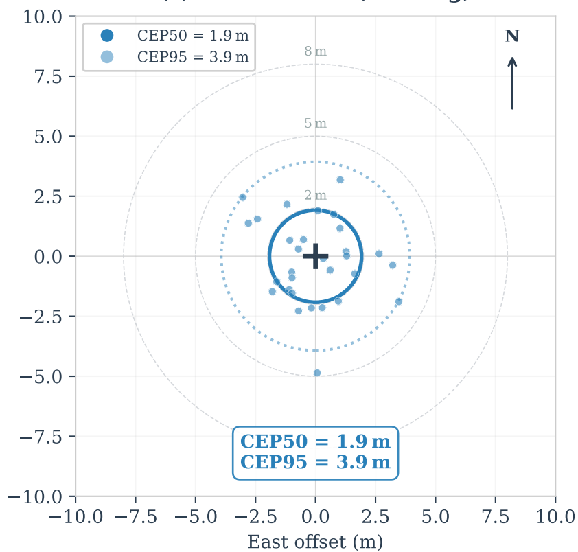
(c) Hover Lock (10 s avg)
