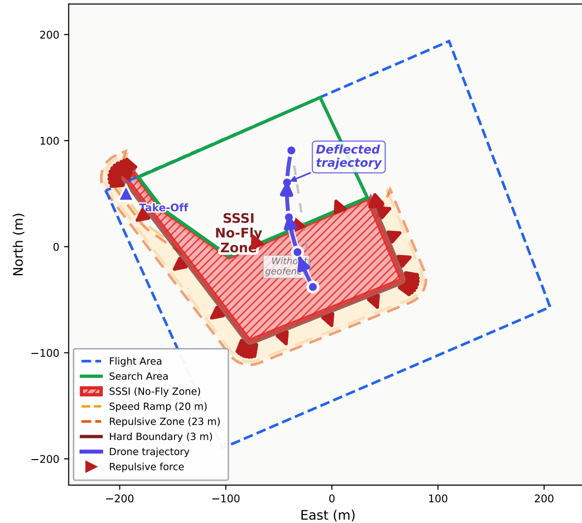
(b) With Three-Layer Geofence Protection
