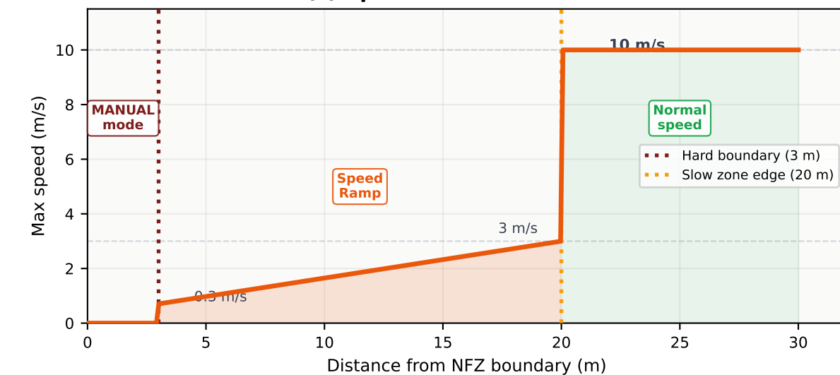
(c) Speed Reduction Profile
