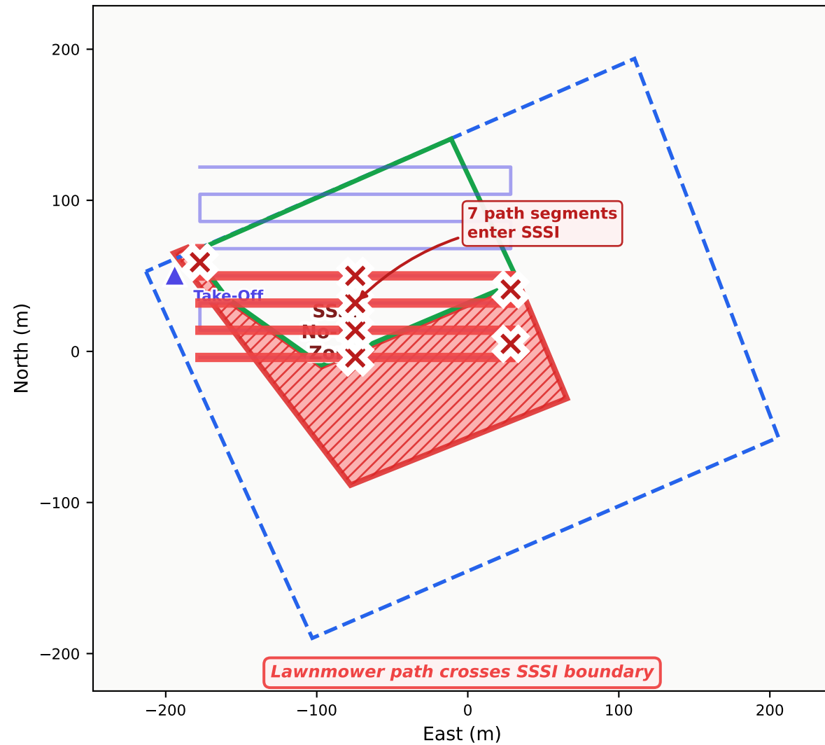
(a) Without Geofence
