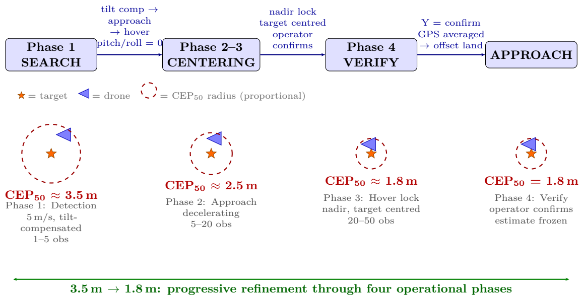
Figure 29: Target GPS estimate accuracy progression through the four-phase detection-to-landing flow. Circle radii are proportional to \text{CEP}_{50} at each phase. Tilt compensation in Phase 1 reduces the initial estimate from \sim 7 \text{ m} (uncompensated) to \sim 3.5 \text{ m} . The combination of continuous approach refinement (Phase 2), hover lock with nadir camera (Phase 3), operator verification with GPS averaging (Phase 4), and spatial deduplication of false positives transforms the initial estimate into a \sim 1.8 \text{ m} final position—a \sim 2\times improvement through operational procedure alone.
