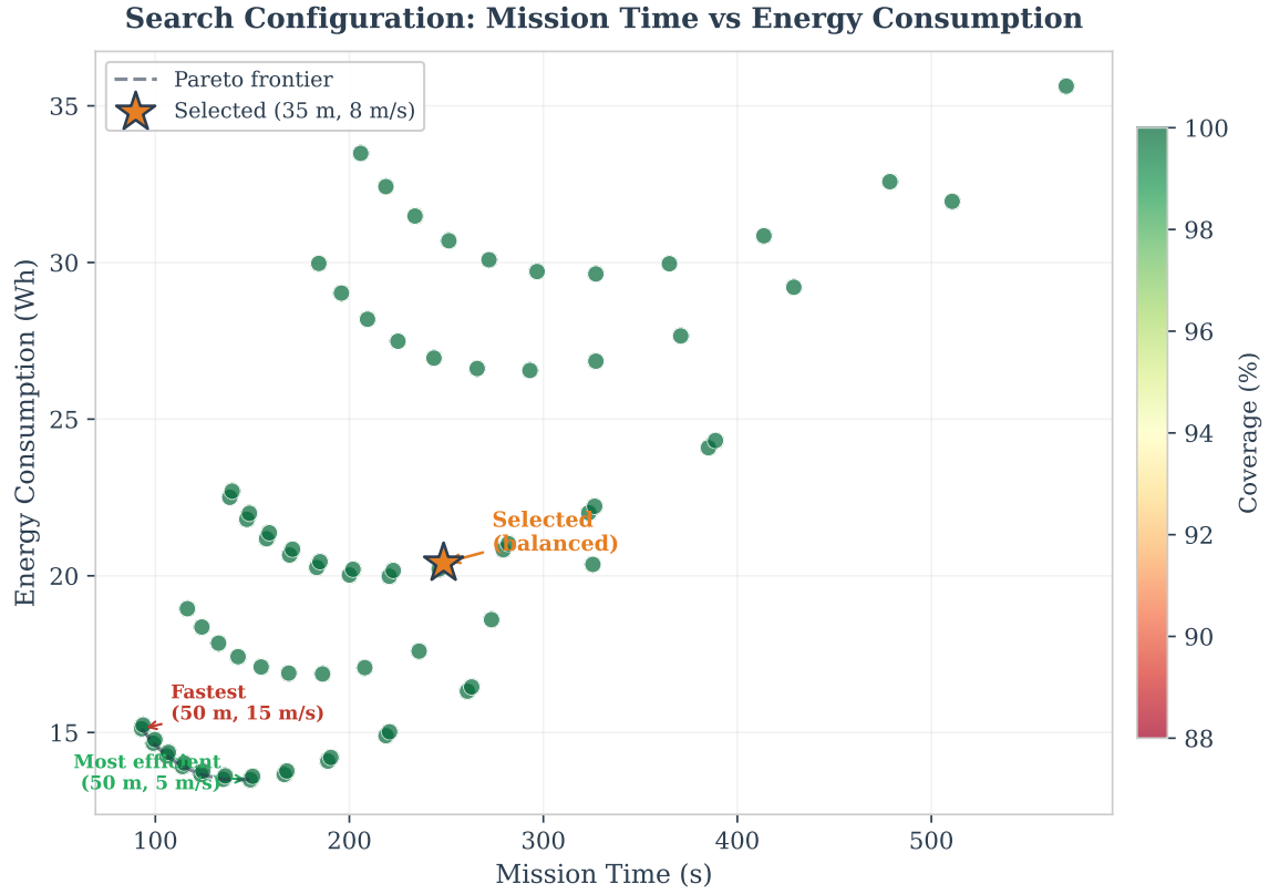
Figure 37: Energy efficiency across the 216-configuration parameter sweep. Lower-energy configurations cluster at high altitude and optimal scan angle; the selected operating point (35 m, 70^\circ , 8 \text{ m s}^{-1} ) trades minimal energy for reliable detection.
