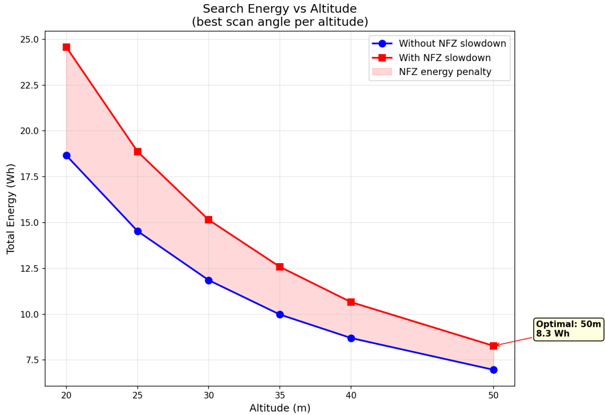
Figure 42: Total search energy versus altitude at the optimal scan angle, with and without NFZ slowdown. The NFZ penalty is most pronounced at 20 m, where several scan lines pass through the slow zone near the SSSI boundary. The shaded region quantifies the additional hover energy incurred by the speed ramp.
