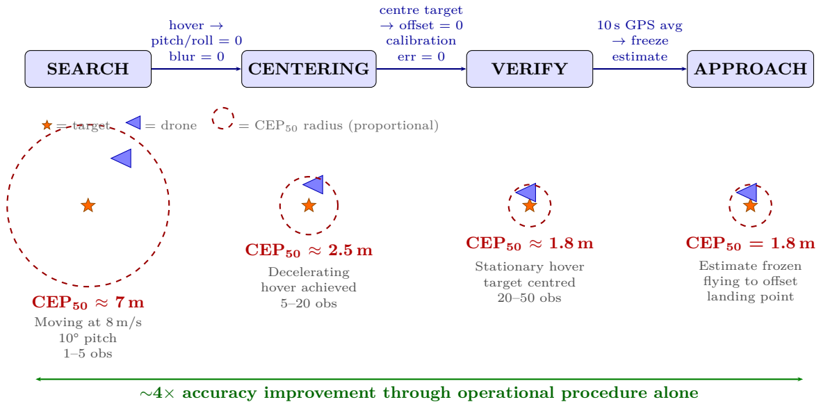
Figure 28: Target GPS estimate accuracy progression through mission phases. Circle radii are proportional to \text{CEP}_{50} at each state. The combination of centering (zero pixel offset), hovering (zero roll/pitch), and GPS averaging transforms a \sim 7 \text{ m} initial estimate into a 1.8 \text{ m} final estimate—a \sim 4\times improvement achieved entirely through operational procedure without additional hardware or software complexity.
