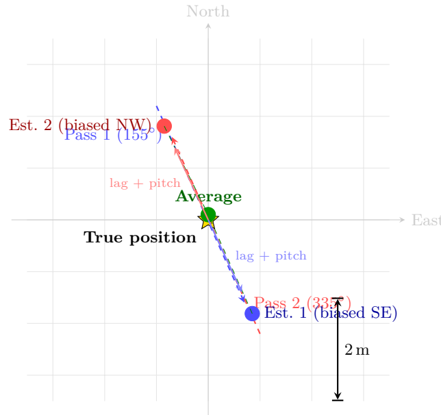
Figure 33: Multi-pass bias cancellation. Pass 1 (heading 155^\circ , blue) biases the GPS estimate south-east; Pass 2 (heading 335^\circ , red) biases it north-west by the same magnitude. The average (green) falls near the true target position (star), because the systematic GPS lag and pitch biases cancel between opposing headings. Only random GPS receiver noise remains.
