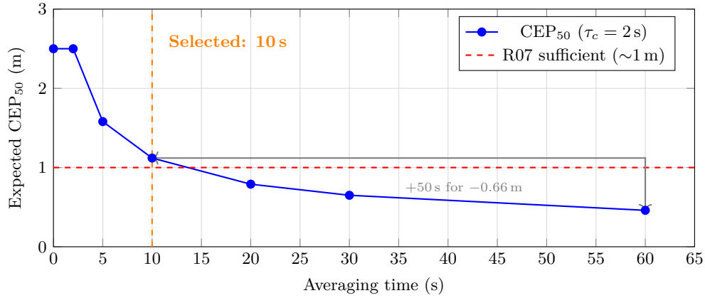
Figure 27: CEP 50 vs. GPS averaging time during stationary hover. The 1/\sqrt{T} convergence means that doubling the averaging time only improves accuracy by \sim 29\% . The 10 s operating point (orange) achieves sub-1.2 m CEP while adding minimal mission time.
