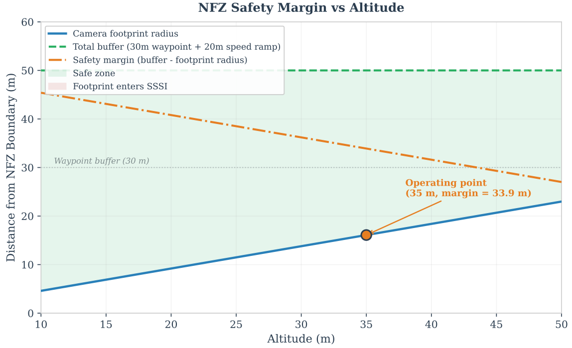
Figure 39: NFZ margin analysis as a function of altitude. The camera footprint radius grows linearly with altitude, but the implemented 50 m total margin maintains a comfortable surplus at all operational altitudes.
