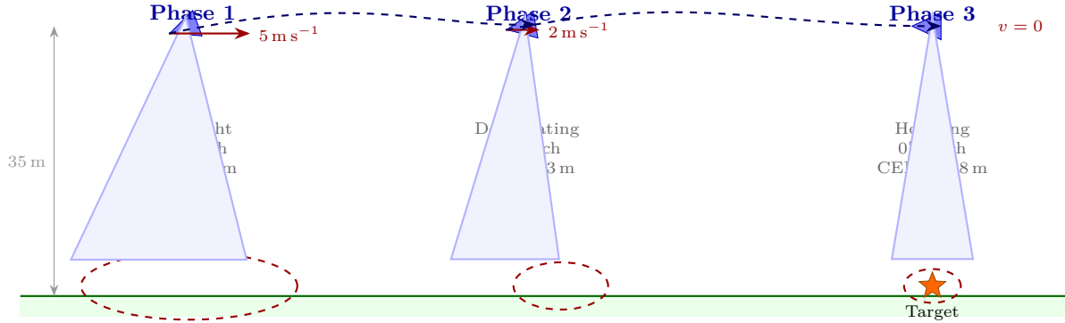
Figure 29: The “creep up” trajectory showing three phases of the two-step detection process. Phase 1: fast flight with tilted camera produces a rough GPS estimate (large error ellipse). Phase 2: the drone decelerates toward the estimate, pitch decreases, and accuracy improves (medium error ellipse). Phase 3: the drone hovers directly above the target with the camera at nadir, producing the precise lock (small error ellipse). Camera cones show the field of view at each phase; the blue triangles represent the drone oriented in its direction of travel.
