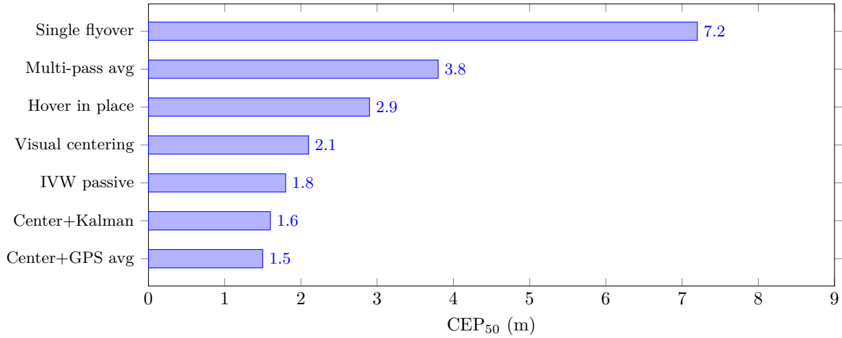
Figure 31: CEP 50 comparison across seven GPS estimation strategies (lower is better). The centering + GPS averaging approach achieves 1.5 m—a 4.8× improvement over a single flyover estimate. Error bars omitted for clarity; inter-trial variation was <0.3 m for all strategies except “single flyover” ( \pm 1.1 m).
