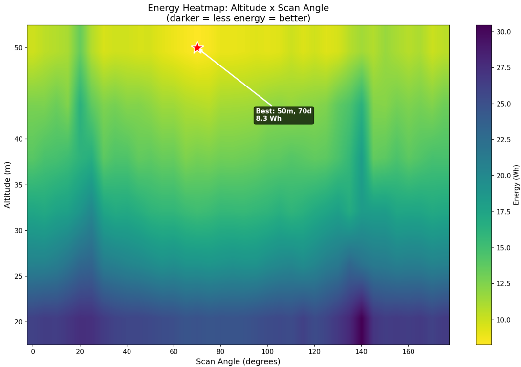
Figure 3: Energy heatmap across 216 altitude–angle configurations. A clear low-energy valley runs through 65\text{--}75^\circ at all altitudes, corresponding to longest-edge alignment. The red star marks the global energy minimum (50 m, 70^\circ ). The selected point (35 m, 70^\circ ) trades 4.4 Wh of energy for a 44% increase in target pixel extent.
