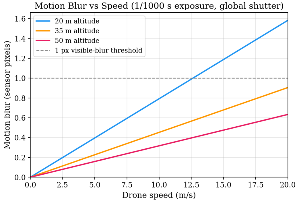
Figure 61: Motion blur vs. drone speed at three altitudes (1/1000 s exposure, global shutter). The grey dashed line marks the 1 px visible-blur threshold.
