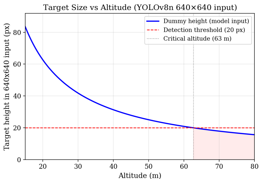
Figure 60: Target height in the 640×640 model input as a function of altitude. The red dashed line marks the 20 px detection threshold; the shaded region indicates unreliable detection.
