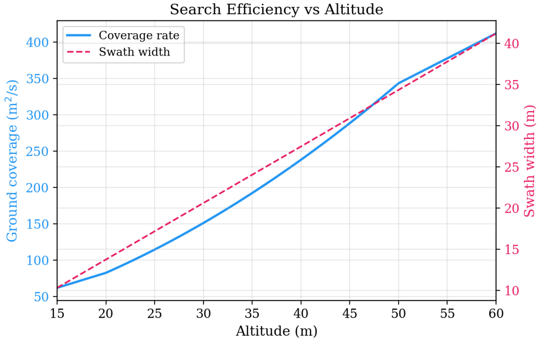
Figure 63: Search efficiency vs. altitude. The solid blue line shows coverage rate ( \text{m}^2/\text{s} ); the dashed pink line shows swath width. Higher altitude improves efficiency at the cost of reduced target pixel size.
