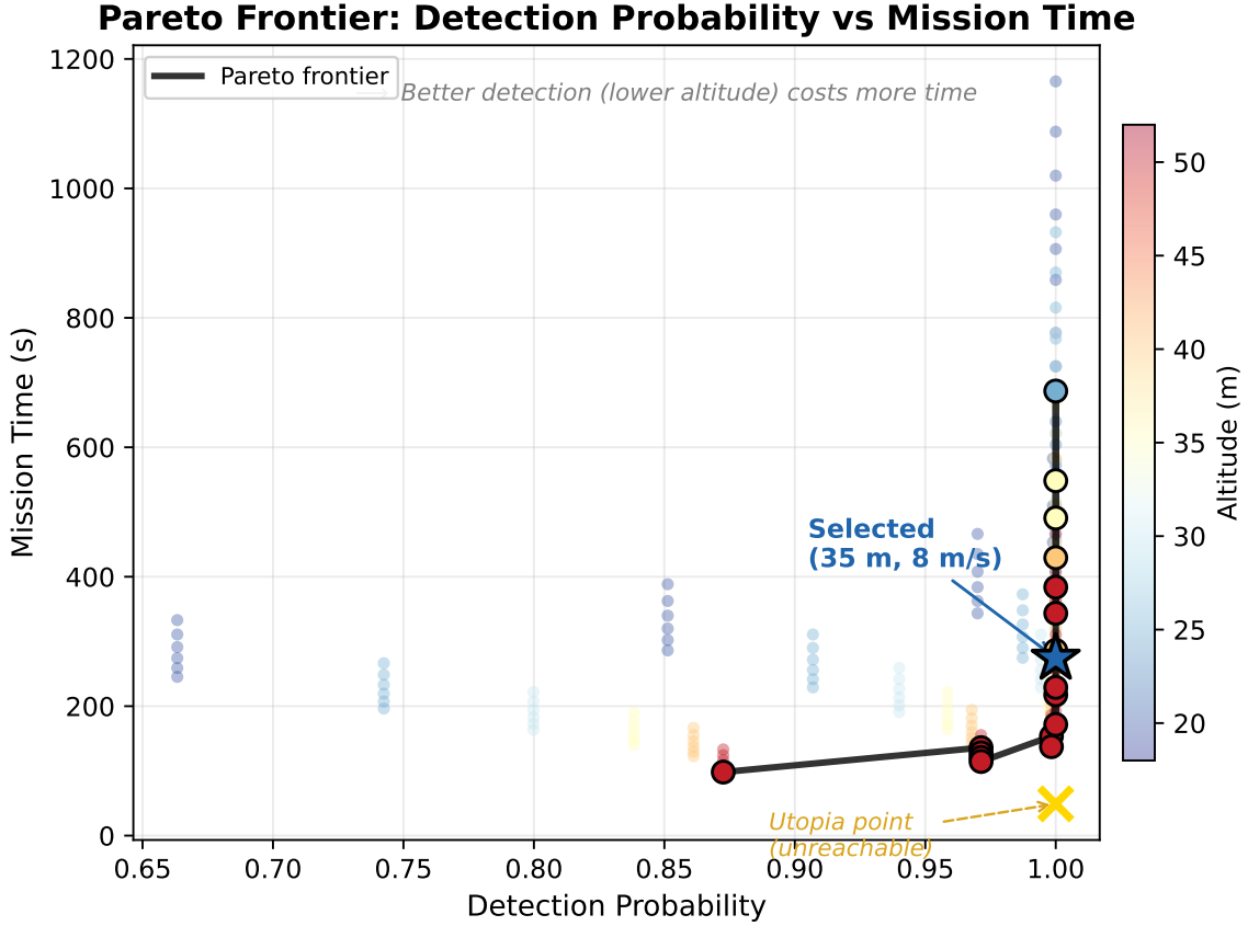
Figure 46: Classical 2D Pareto curve: detection probability vs mission time. Each dot represents one of the 216 swept configurations, coloured by altitude. The Pareto frontier connects non-dominated solutions. The selected operating point (35 m, 8 m/s) sits at the knee of the curve.
