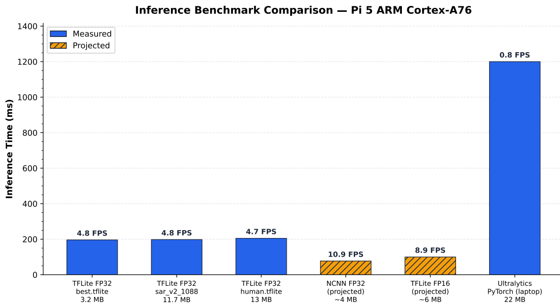
Figure 24: Inference backend comparison on Raspberry Pi 5 for YOLOv8n ( 640 \times 640 input). TFLite with XNNPACK provides the measured production baseline at 4.8FPS; NCNN and FP16 projections indicate viable paths to real-time performance.
