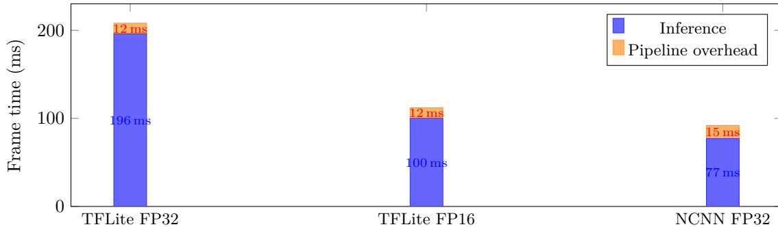
Figure 50: Frame time decomposition: inference vs. pipeline overhead for each backend. As raw inference latency decreases, overhead transitions from negligible (5.8% for TFLite FP32) to significant (16.3% for NCNN).
