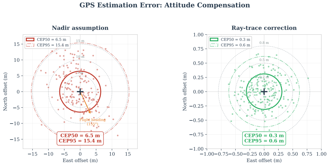
Figure 37: GPS target estimate scatter before and after attitude compensation at 35 m altitude. Without compensation (left), forward-flight pitch introduces a systematic along-track bias of \sim 6.2 m. With compensation (right), the ray-trace correction reduces the scatter to \sim 0.3 m, limited by telemetry noise. Data from the 1440-test verification sweep described above.
