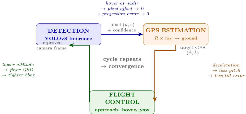
Figure 33: Cooperative vision-flight feedback loop. Detection produces a pixel coordinate, GPS estimation projects it to the ground, and flight control steers the drone toward the target. Crucially, flying closer improves the next detection: lower altitude yields finer GSD, deceleration reduces pitch-induced tilt error, and hovering at nadir drives the pixel offset—and therefore all multiplicative projection errors—toward zero. The cycle repeats until convergence, typically within 15–20 s.
