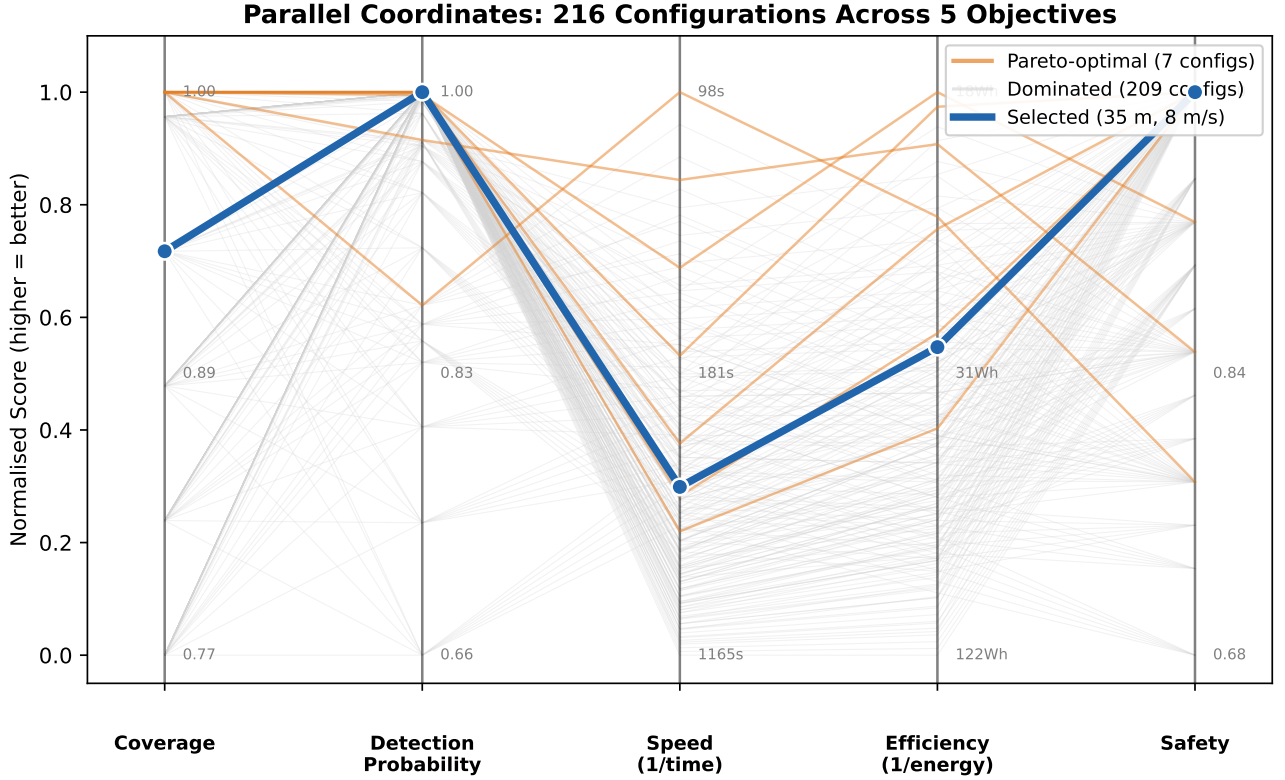
Figure 60: Parallel coordinates plot showing all five objectives simultaneously without dimensional projection. Orange lines indicate the seven Pareto-optimal configurations; the selected configuration (thick blue) achieves balanced performance across all axes. This representation reveals that the selected point trades speed and energy efficiency for superior detection and safety.
