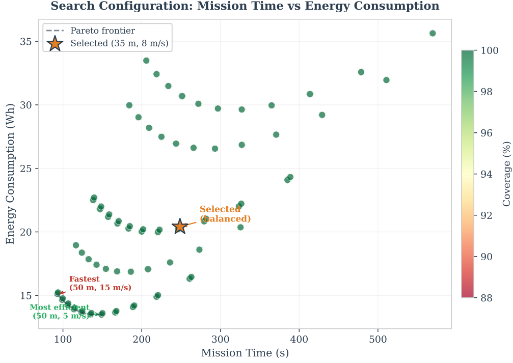
Figure 62: Energy efficiency across the operating range. The search phase consumes only 10.9% of battery capacity at the selected operating point, leaving ample margin for transit, descent phases, and RTL.
