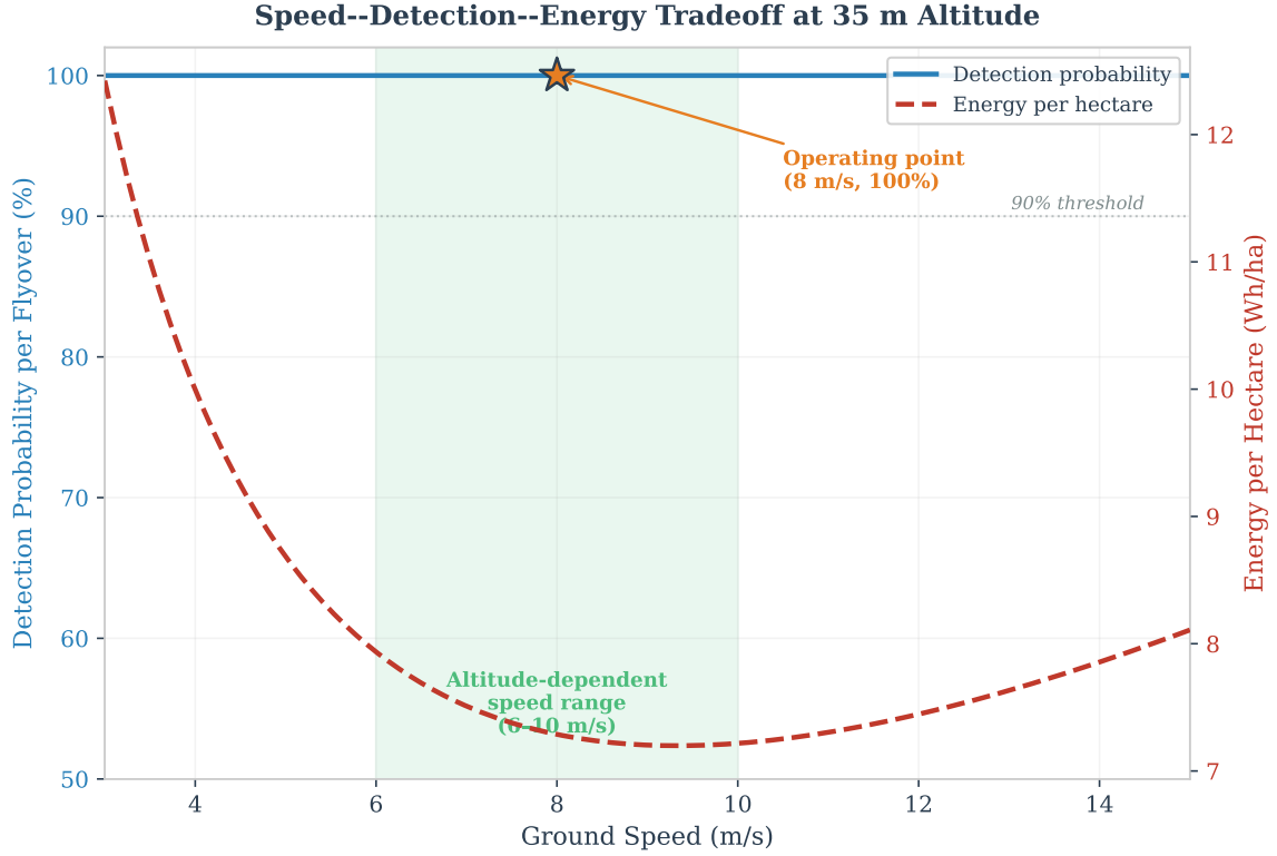
Figure 43: Speed–detection–energy trade-off at 35 m altitude. Detection probability remains above 99.6% across all speeds; the binding constraint is energy consumption and NFZ margin rather than detection reliability.
