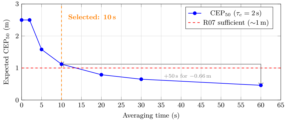
Figure 29: CEP 50 vs. GPS averaging time during stationary hover. The 1/\sqrt{T} convergence means that doubling the averaging time only improves accuracy by \sim 29\% . The 10 s operating point (orange) achieves sub-1.2 m CEP while adding minimal mission time.
