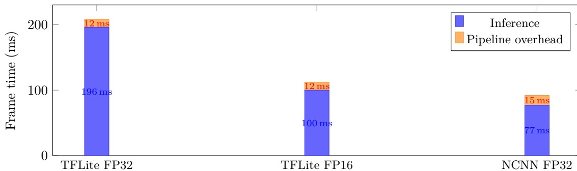
Figure 39: Frame time decomposition: inference vs. pipeline overhead for each backend. As raw inference latency decreases, overhead transitions from negligible (5.8% for TFLite FP32) to significant (16.3% for NCNN).
