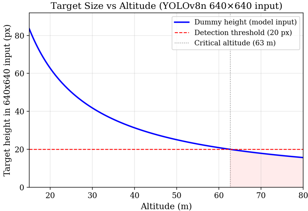
Figure 72: Target height in the 640 \times 640 model input as a function of altitude. The red dashed line marks the 20 px detection threshold; the shaded region indicates unreliable detection.
