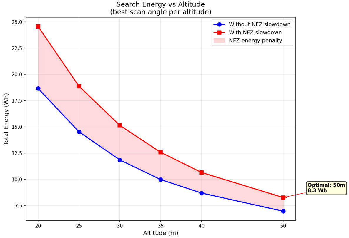
Figure 45: Total search energy versus altitude at the optimal scan angle, with and without NFZ slowdown. The NFZ penalty is most pronounced at 20 m, where several scan lines pass through the slow zone near the SSSI boundary. The shaded region quantifies the additional hover energy incurred by the speed ramp.
