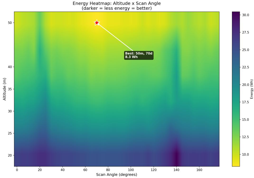
Figure 53: Energy heatmap across 216 altitude–angle configurations. A clear low-energy valley runs through 65\text{--}75^\circ at all altitudes, corresponding to longest-edge alignment. The red star marks the global energy minimum ( 50\text{ m}, 70^\circ ). The selected point ( 35\text{ m}, 70^\circ ) trades 4.4\text{ Wh} of energy for a 44% increase in target pixel extent.
