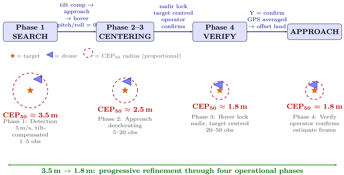
Figure 30: Target GPS estimate accuracy progression through the four-phase detection-to-landing flow. Circle radii are proportional to CEP 50 at each phase. Tilt compensation in Phase 1 reduces the initial estimate from ~7 m (uncompensated) to ~3.5 m. The combination of continuous approach refinement (Phase 2), hover lock with nadir camera (Phase 3), operator verification with GPS averaging (Phase 4), and spatial deduplication of false positives transforms the initial estimate into a ~1.8 m final position—a ~2× improvement through operational procedure alone.
