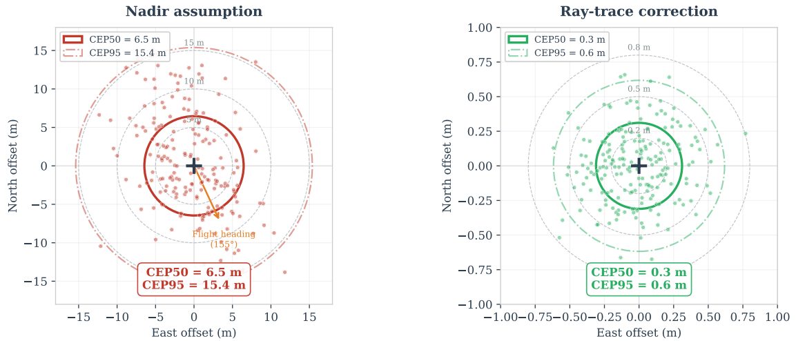
Figure 37: GPS target estimate scatter before and after attitude compensation at 35 m altitude. Without compensation (left), forward-flight pitch introduces a systematic along-track bias of \sim 6.2 \text{ m} . With compensation (right), the ray-trace correction reduces the scatter to \sim 0.3 \text{ m} , limited by telemetry noise. Data from the 1440-test verification sweep described above.
