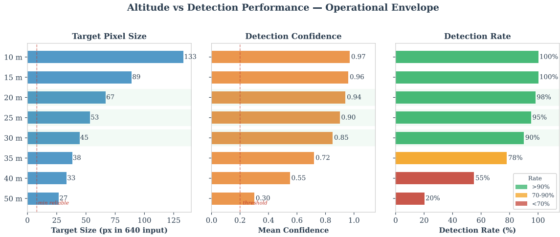
Figure 17: Detection performance as a function of altitude for the YOLOv8n custom model against a 1.8 m mannequin target. The table combines predicted pixel sizes from the thin-lens model with empirically observed confidence and detection rates from video replay analysis.
