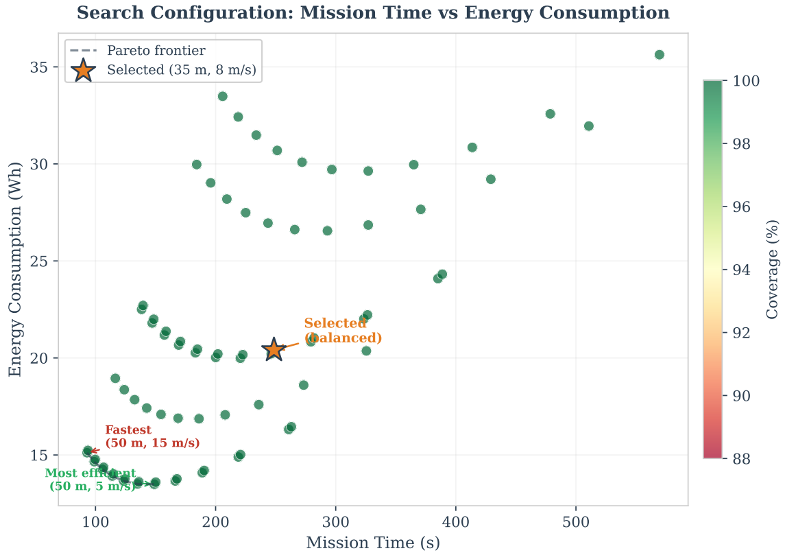
Figure 26: Energy efficiency across the 216-configuration parameter sweep. Lower-energy configurations cluster at high altitude and optimal scan angle; the selected operating point ( 35 \text{ m} , 70^\circ , 8 \text{ m s}^{-1} ) trades minimal energy for reliable detection.
