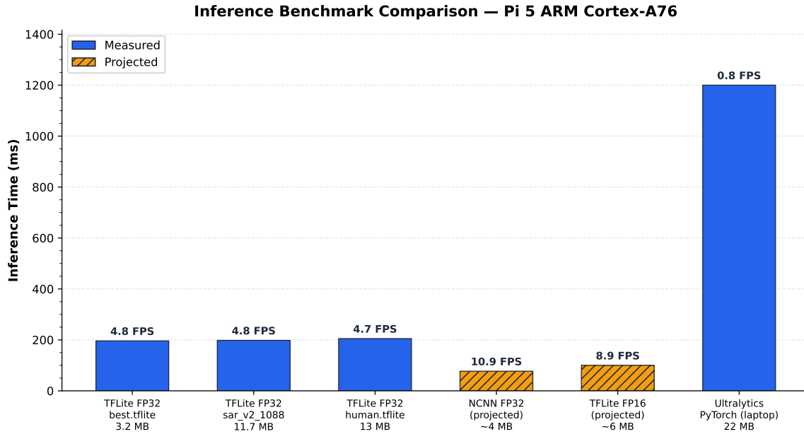
Figure 16: Inference backend comparison on Raspberry Pi 5 for YOLOv8n ( 640 \times 640 input). TFLite with XNNPACK provides the measured production baseline at 4.8 FPS; NCNN and FP16 projections indicate viable paths to real-time performance.
