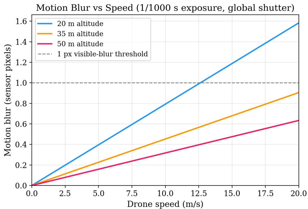
Figure 38: Motion blur vs. drone speed at three altitudes (1/1000 s exposure, global shutter). The grey dashed line marks the 1 px visible-blur threshold.
