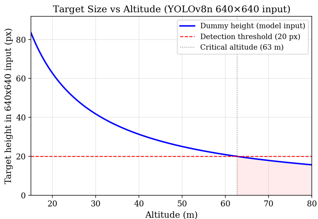
Figure 37: Target height in the 640×640 model input as a function of altitude. The red dashed line marks the 20 px detection threshold; the shaded region indicates unreliable detection.
