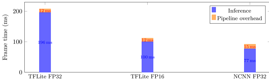
Figure 25: Frame time decomposition: inference vs. pipeline overhead for each backend. As raw inference latency decreases, overhead transitions from negligible (5.8% for TFLite FP32) to significant (16.3% for NCNN).
