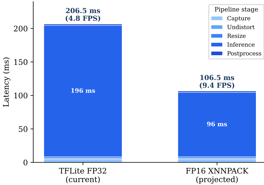
Figure 22: Latency breakdown of the detection pipeline. Model inference (XNNPACK, 4-thread) accounts for 94% of total latency; all other stages are negligible in comparison.
