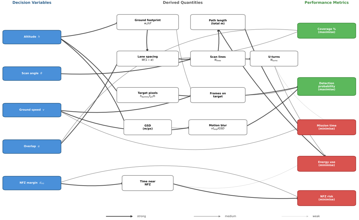
Figure 34: Optimisation variable dependency network. Decision variables (blue) cascade through derived quantities (white) to performance metrics (green/red). Arrow thickness indicates influence strength.
