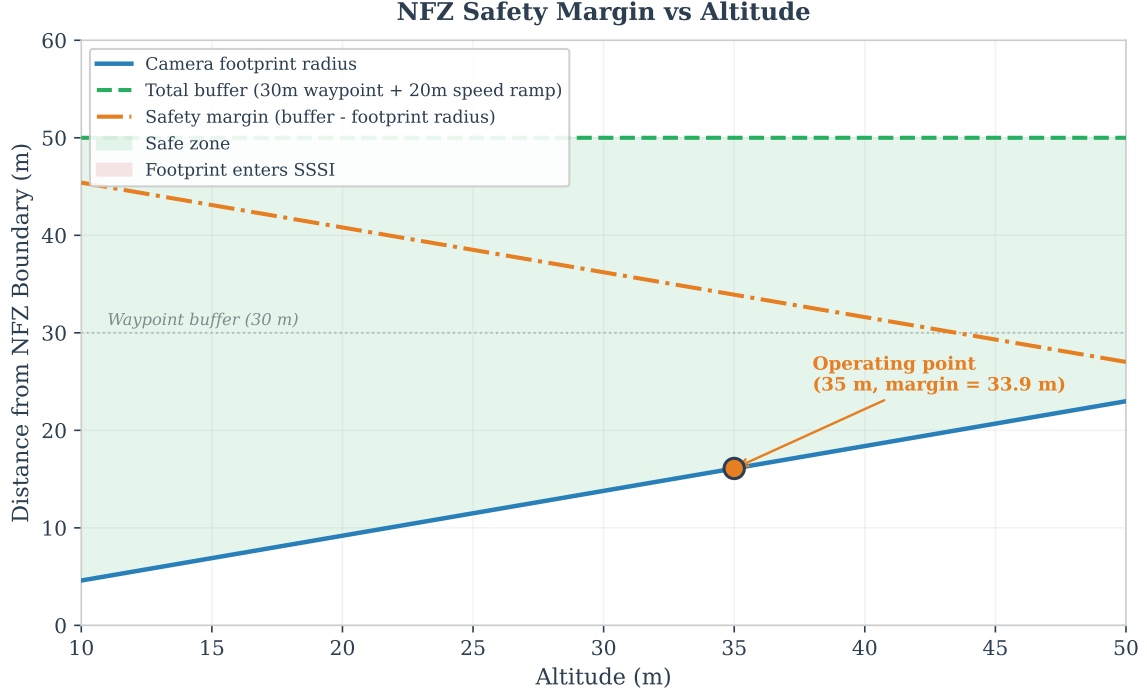
Figure 28: NFZ margin analysis as a function of altitude. The camera footprint radius grows linearly with altitude, but the implemented 50 m total margin maintains a comfortable surplus at all operational altitudes.
