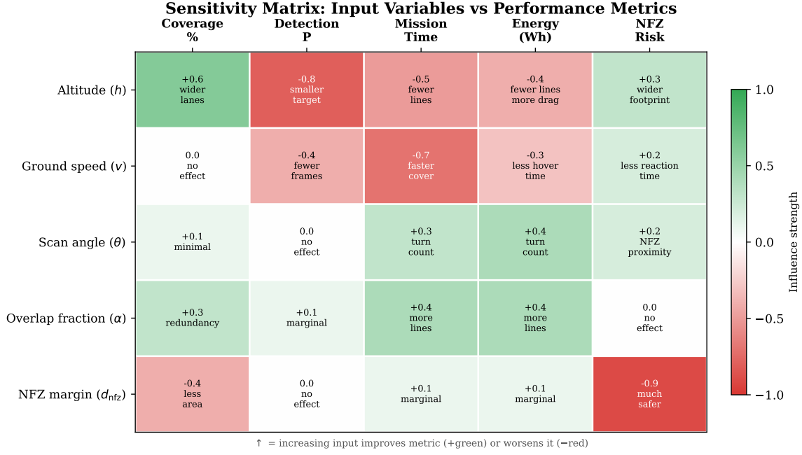
Figure 35: Sensitivity matrix showing the influence of each input parameter on every derived quantity. Darker cells indicate stronger coupling, revealing which measurements most critically affect mission performance.
