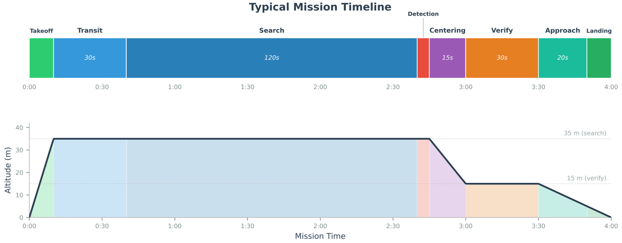
Figure 7: Mission timeline showing state transitions during a simulated end-to-end SAR mission. The horizontal axis represents elapsed time; coloured blocks indicate active states.
