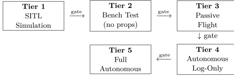
Figure 13: Tier progression. Each arrow represents a gate: the downstream tier is blocked until all upstream tests pass.
