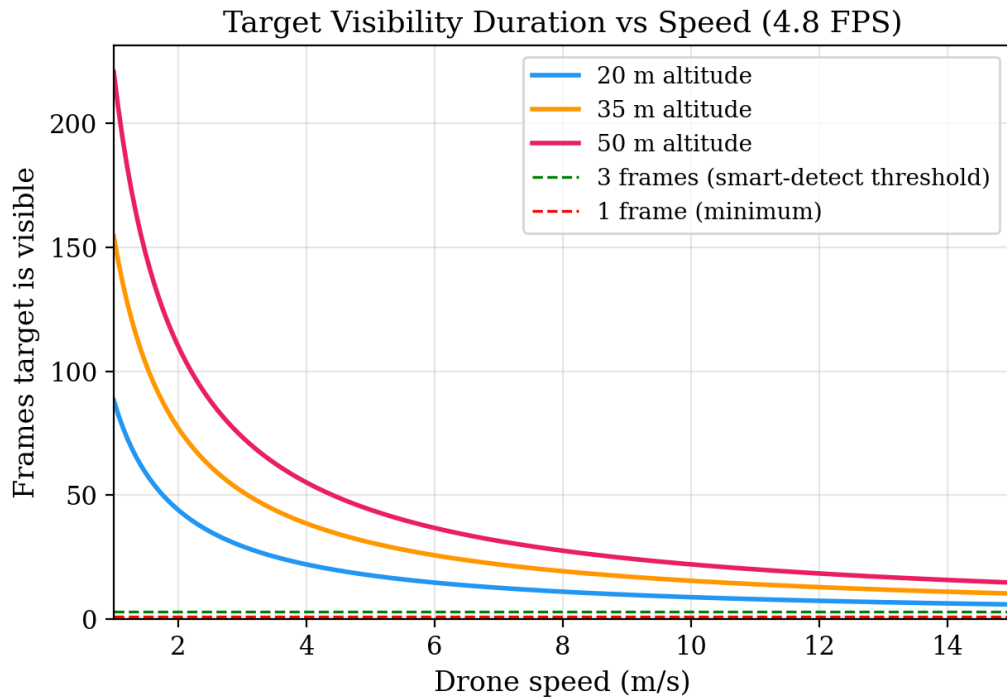
Figure 58: Frames the target remains visible vs. drone speed at three altitudes (4.8 FPS). The green and red dashed lines mark the 3-frame smart-detect threshold and 1-frame minimum, respectively.
