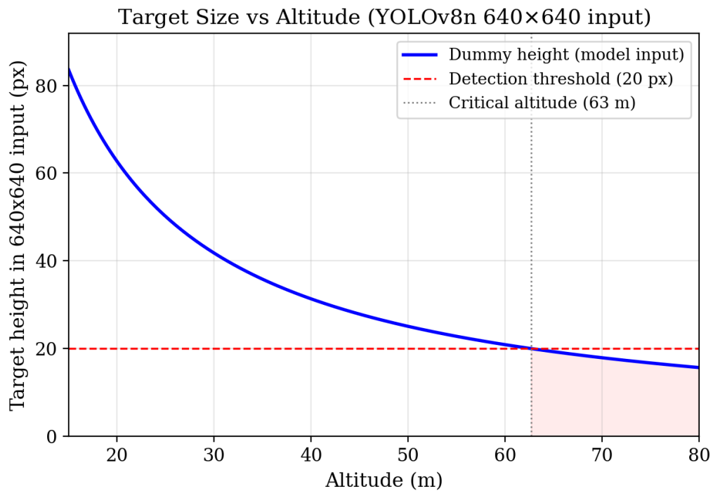
Figure 56: Target height in the 640×640 model input as a function of altitude. The red dashed line marks the 20 px detection threshold; the shaded region indicates unreliable detection.
