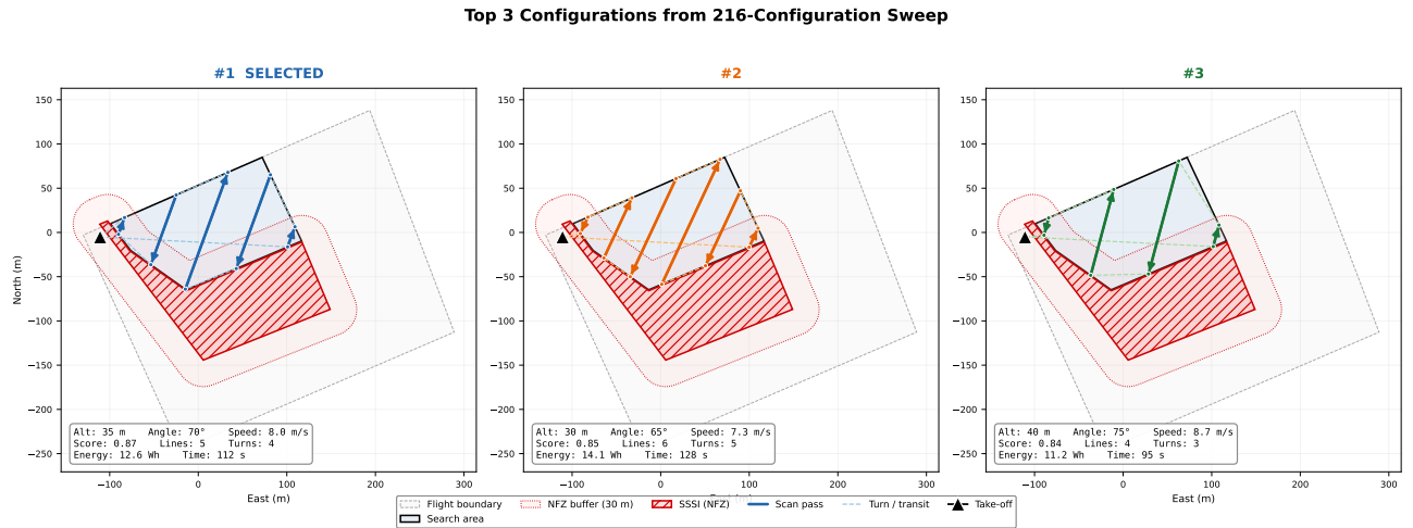
Figure 35: Top three energy-ranked search configurations overlaid on the AENGM0074 survey polygon. Each panel shows the lawnmower pattern at the corresponding altitude and scan angle, with path length, scan line count, and energy annotated. The selected operating point (35 m, 70°) balances detection reliability against the energy savings of higher altitudes.
