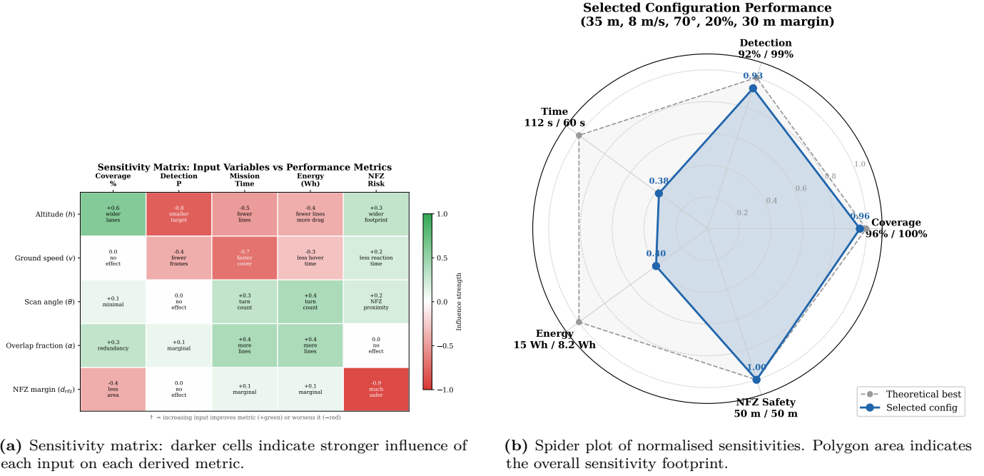
Figure 44: Complementary sensitivity visualisations at the selected operating point (35 m, 70°, 8 m s -1 ).
