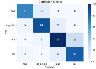
Fig. 5. Confusion Matrix of Event Classification Model
