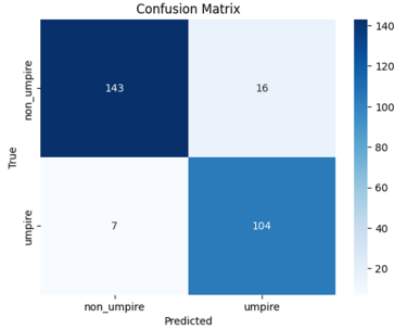
Fig. 3. Confusion Matrix of Umpire Detection Model
