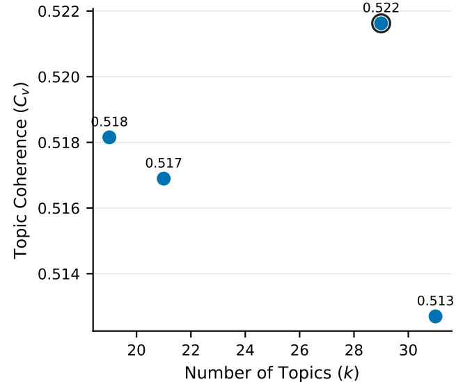
(a) LDA
