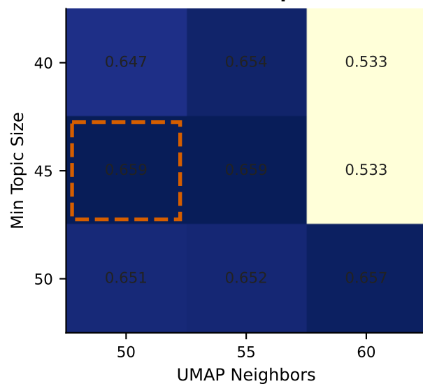
(c) BERTopic
