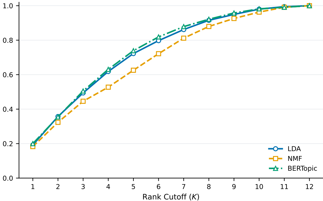
Cumulative Relevant Group Fraction
