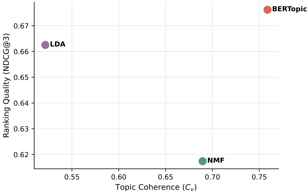
Topic Coherence vs. Downstream Performance
