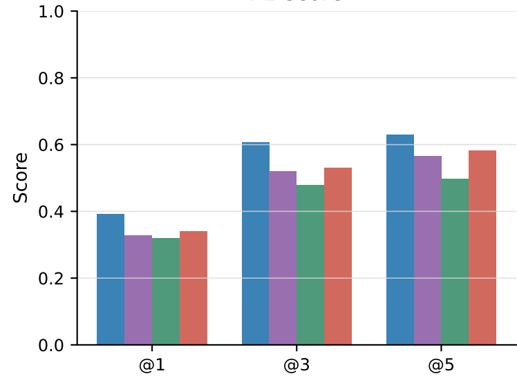
F1-score
