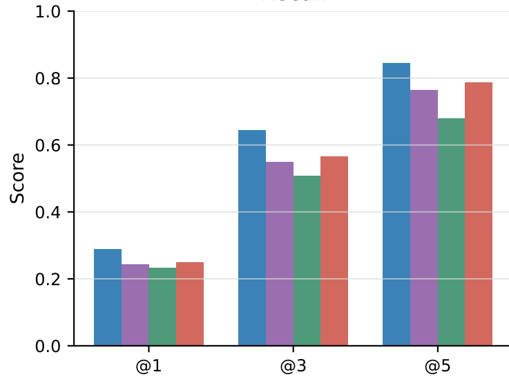
Recall
