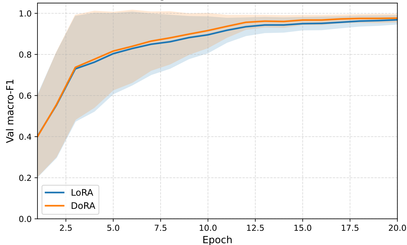
Convergence (mean \pm std, 3 seeds)
