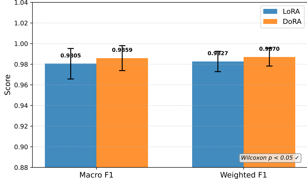
Final Test Metrics (mean \pm std, 3 seeds)
