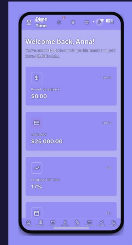
Live dashboard
