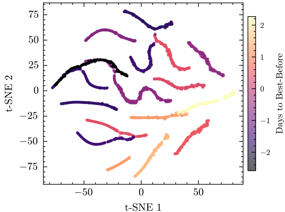
Sensor A, t-SNE
