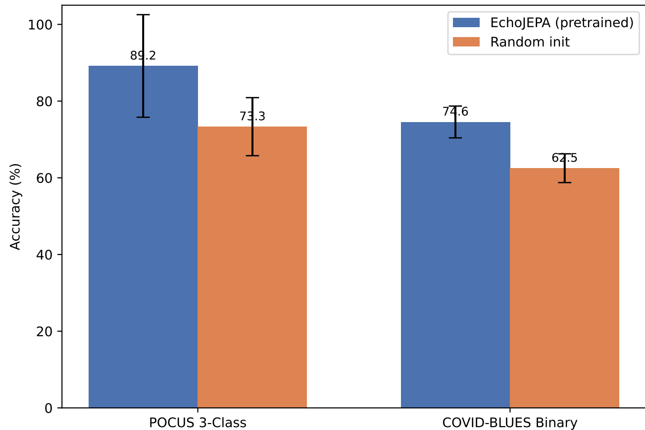
5-Fold CV: Pretrained vs Random Init
