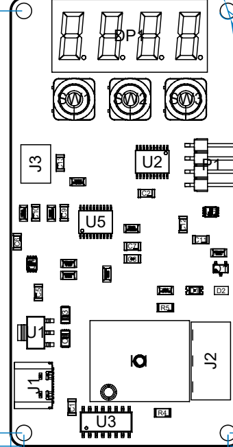
View from Top side (Scale 1:1)
