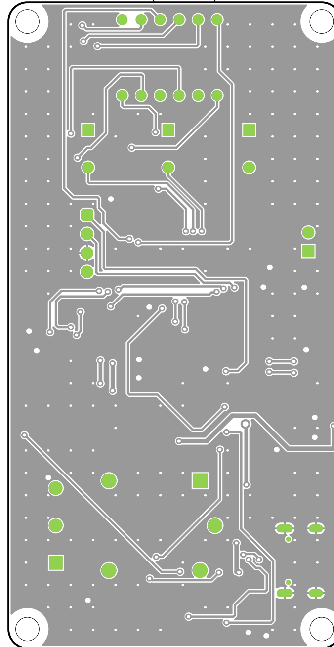
View from Bottom side (Scale 2:1)
