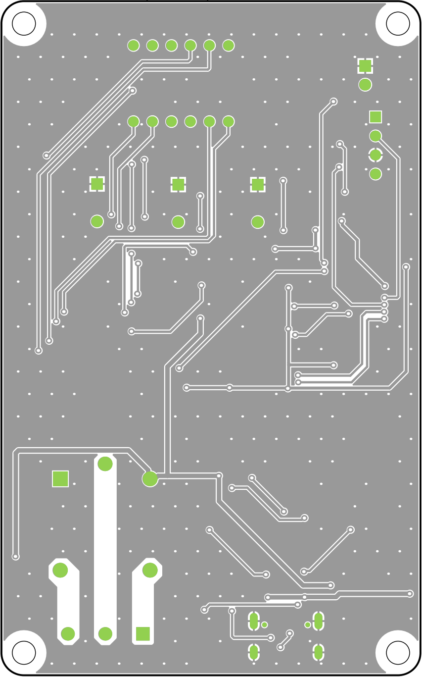
View from Bottom side (Scale 2:1)
