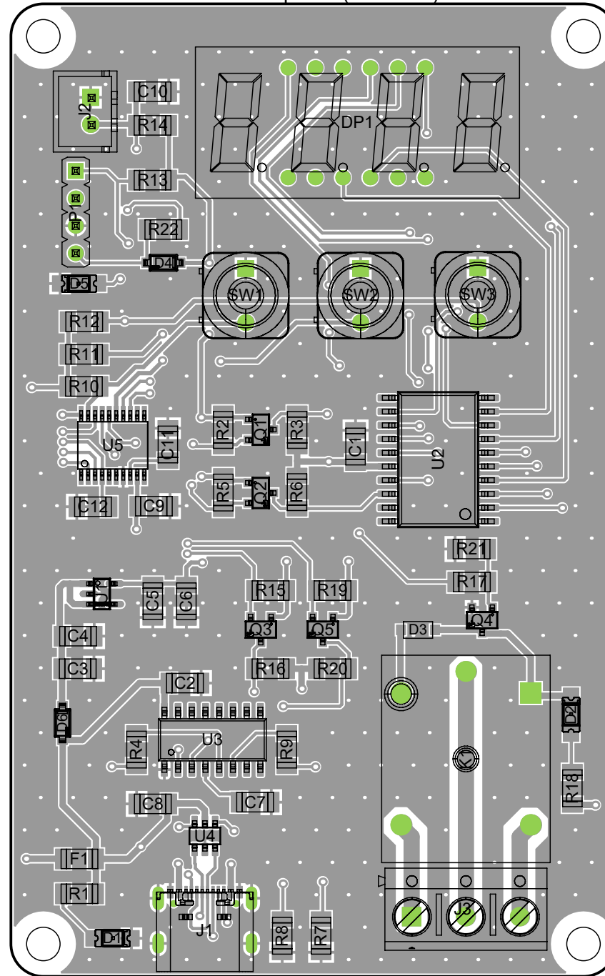
View from Top side (Scale 2:1)
