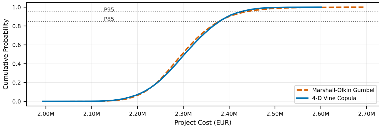
(a) Cost CDF: Vine Copula vs. Marshall-Olkin Gumbel
