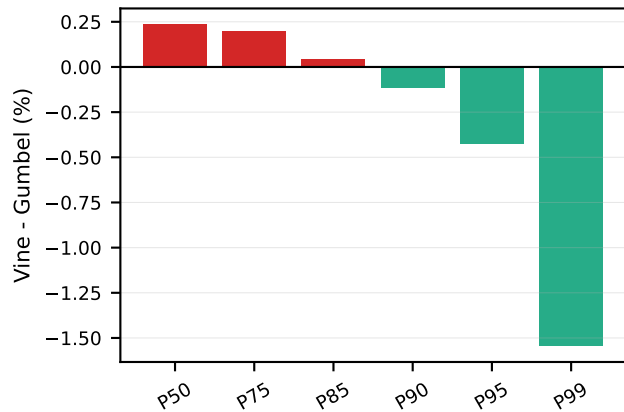
(c) Relative Difference (Vine vs. Gumbel)
