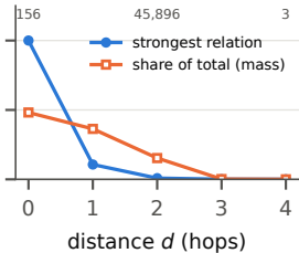
Wiki-Elec relations
