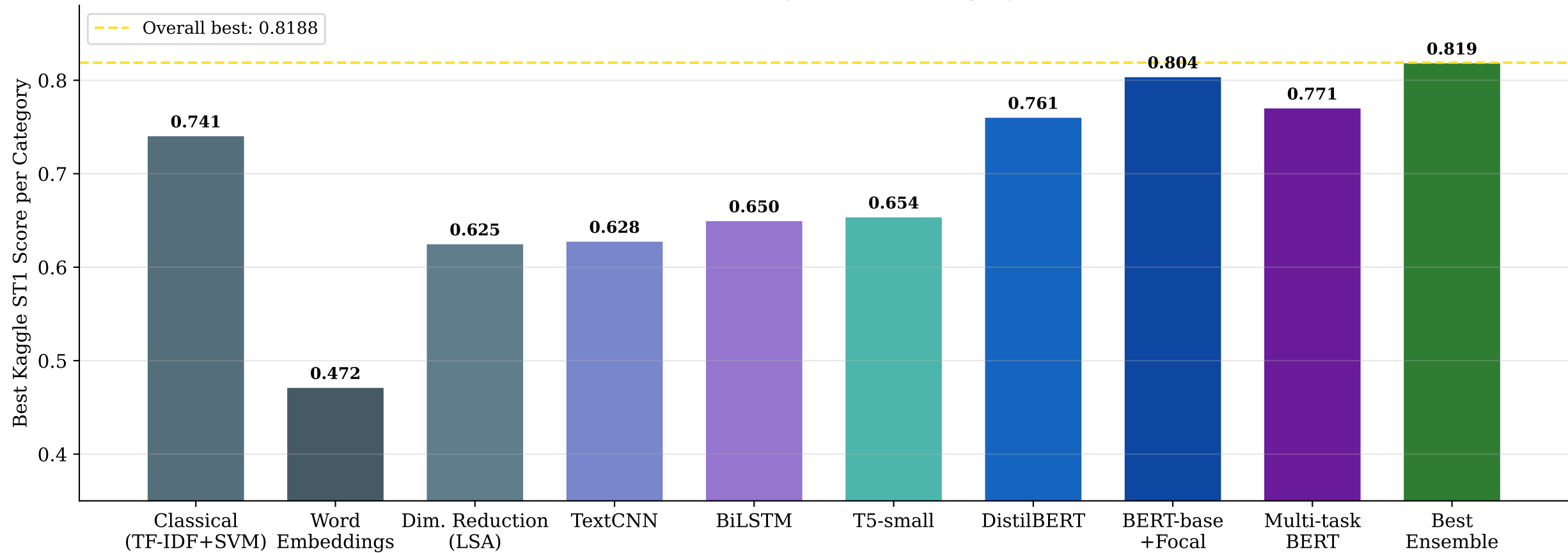
Best Score by Method Category
