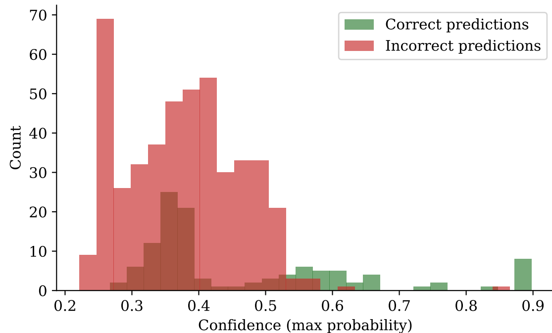
Confidence Distribution — BERT-base + Focal (Hazard)
