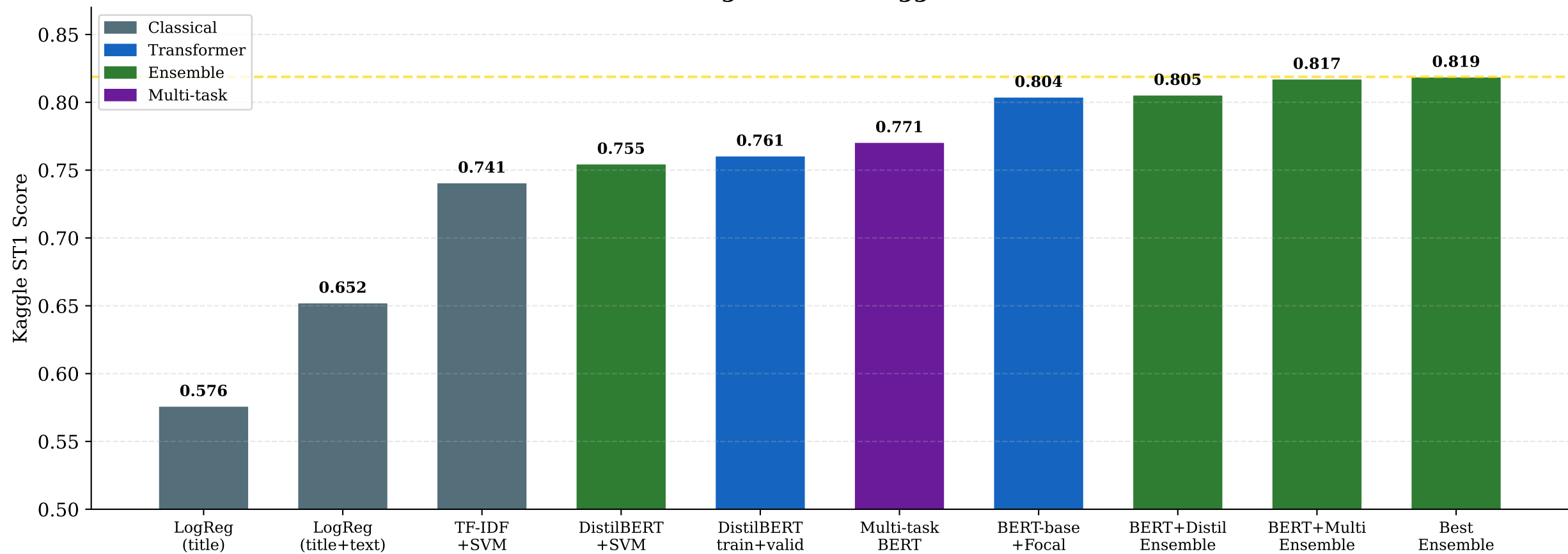
Method Progression — Kaggle ST1 Score
