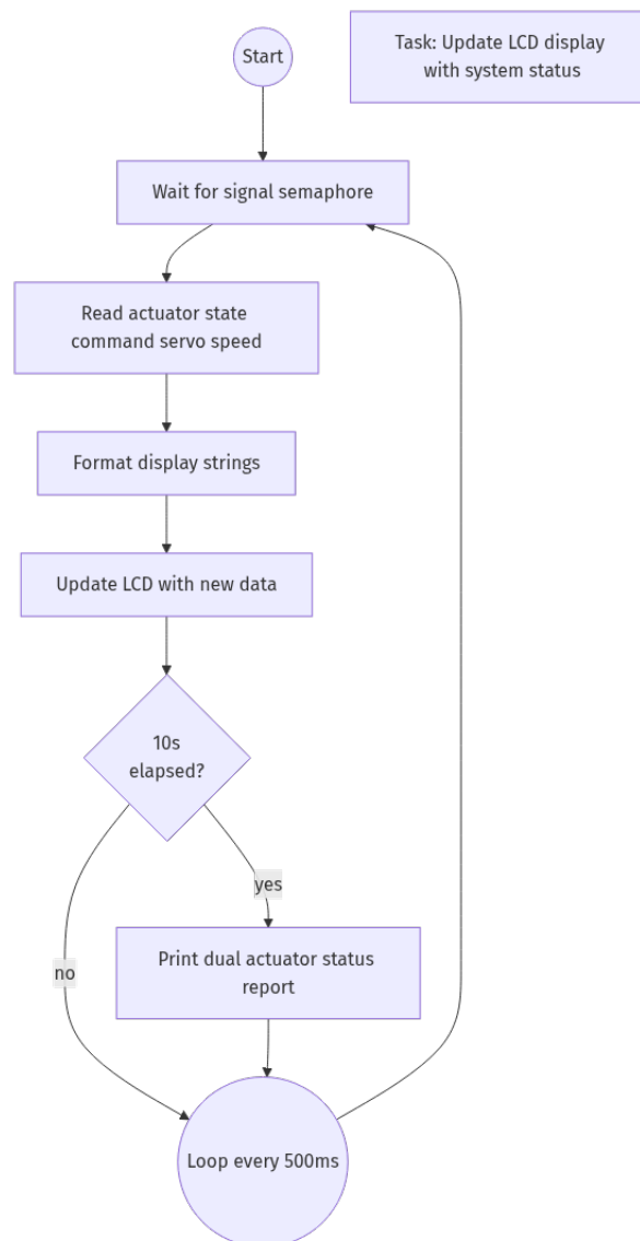
Рис. 7: Activity Diagram - Display Update Task
