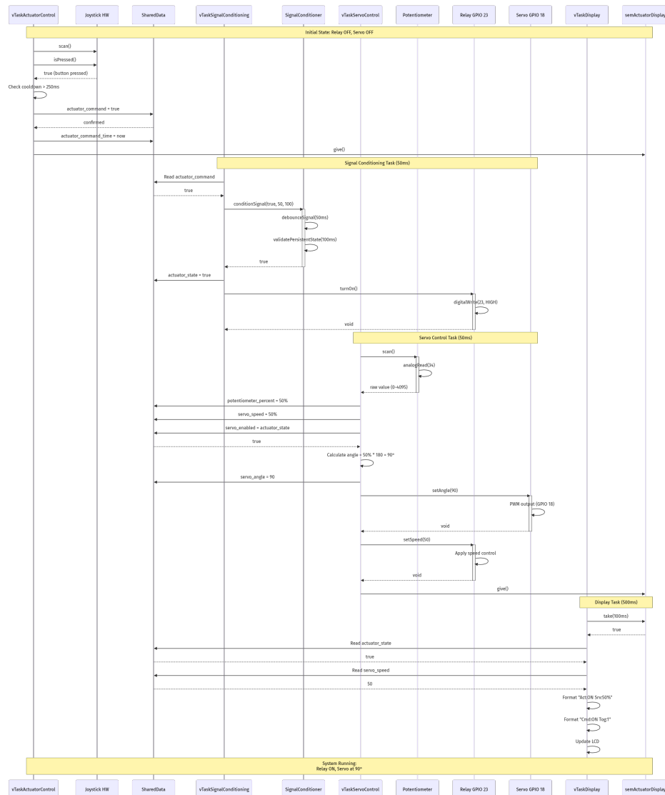
Рис. 9: Sequence Diagram - Dual Actuator Control Flow
