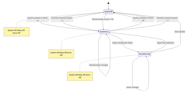
Рис. 10: State Machine - System States and Transitions
