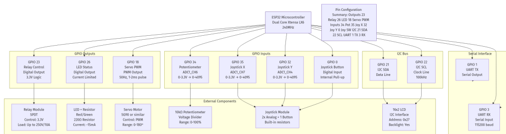
Рис. 16: Hardware Connection Diagram - Dual Actuator Control System
